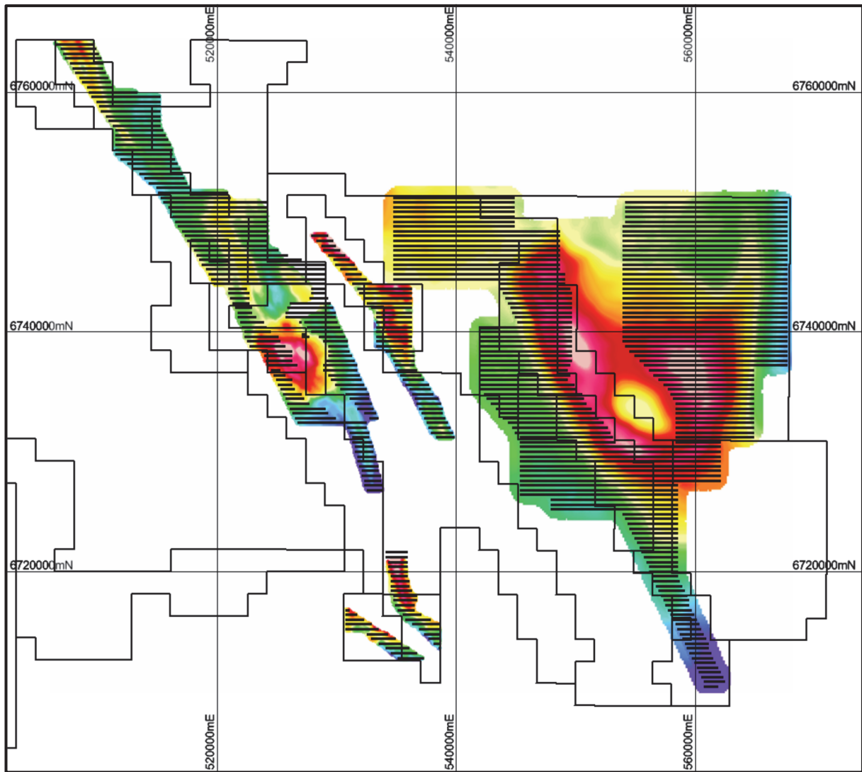
Figure 2 – the preliminary Bouguer gravity data (linear stretch optimised by area) from the extended gravity survey shown over a tenement outline of St George’s Project. The survey has been arranged by Newexco with field work completed by Daishsat Pty Ltd. The survey grid is 200m x 400m, with 10,414 stations completed.
