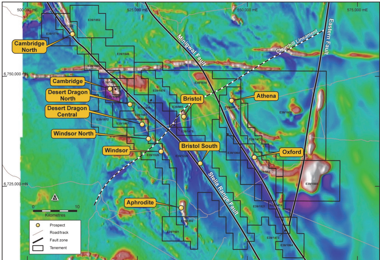
Figure 3 – the high priority prospects and tenement outline at St George’s Project shown over magnetics.
