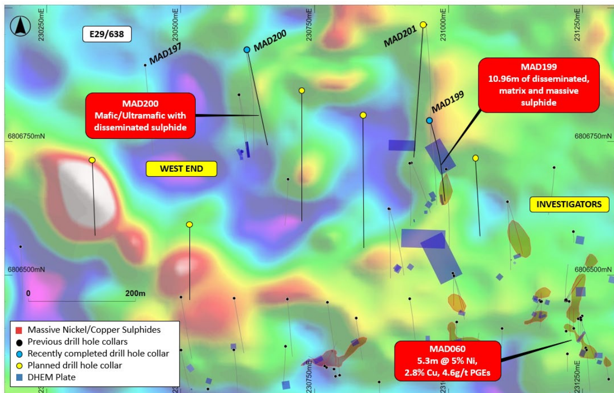
Figure 1 – map of Investigators and West End showing drilling, untested DHEM plates and known massive nickel-copper sulphide occurrences overlaying newly acquired Gravity image (Residual 1VD).
