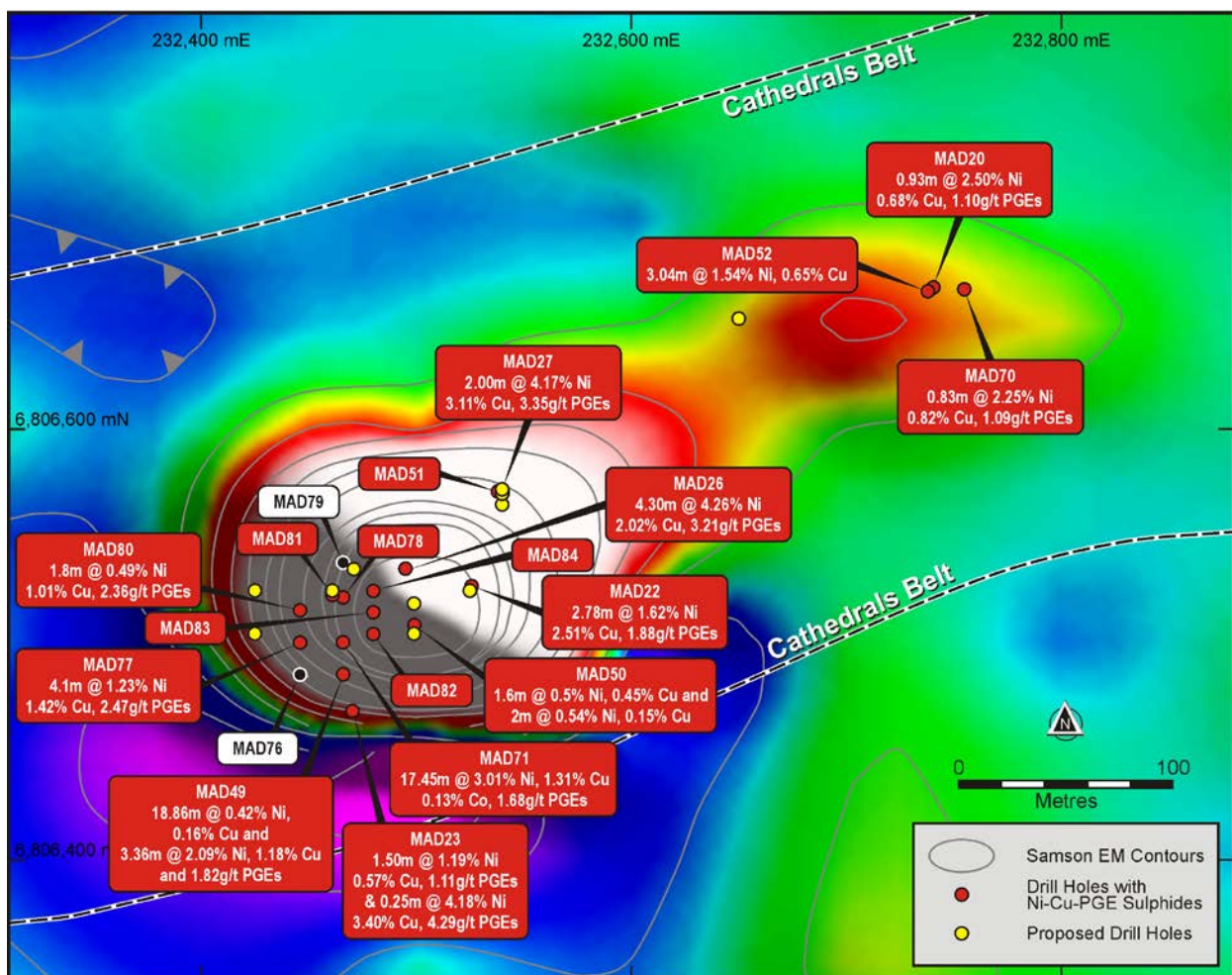
Figure 1 – a plan view of the Stricklands Prospect with drill hole collar locations (completed and planned) over the large SAMSON total field EM anomaly (white/red colours). The SAMSON EM image is shown in Channel 18 (44ms). The contours shown are 0.05pT/A which highlight the stronger electromagnetic field over the Stricklands Prospect.
