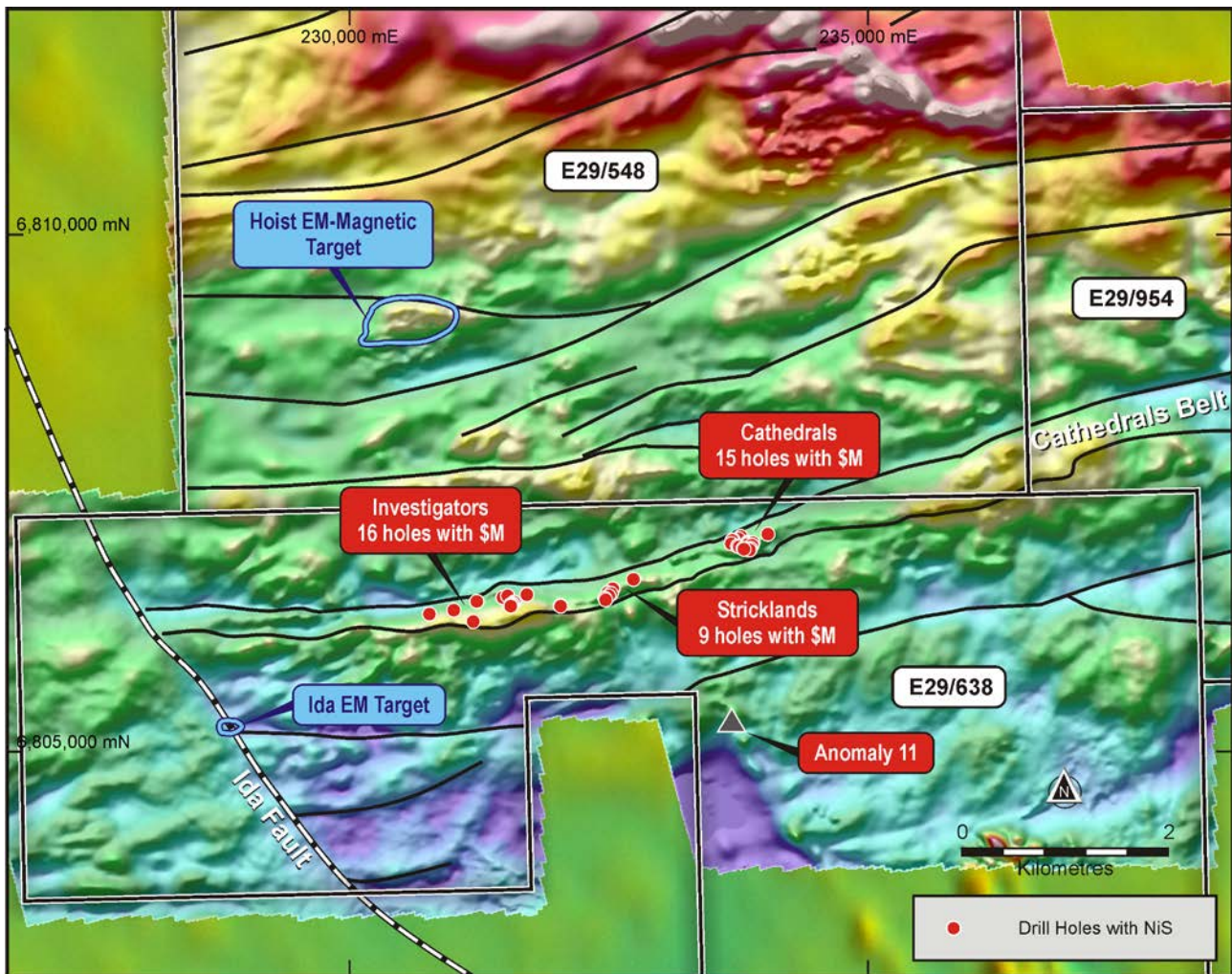
Figure 2 – a map of the Cathedrals Belt (against high resolution Total Magnetic Intensity) showing the new regional targets as well as the multiple intersections of massive nickel-copper-cobalt-PGE sulphides (“$M”) at Investigators, Stricklands and Cathedrals which have established recurrent high grade mineralisation over a strike length of 3.5km. The high resolution magnetic data is set against TMI RTP magnetics from GSWA aeromagnetic surveys.
