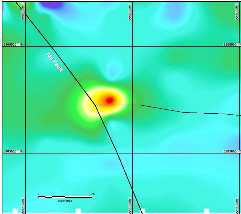
Figure 3 – the SAMSON EM image for the EM target on the Ida Fault shown in Channel 18 (44ms).
