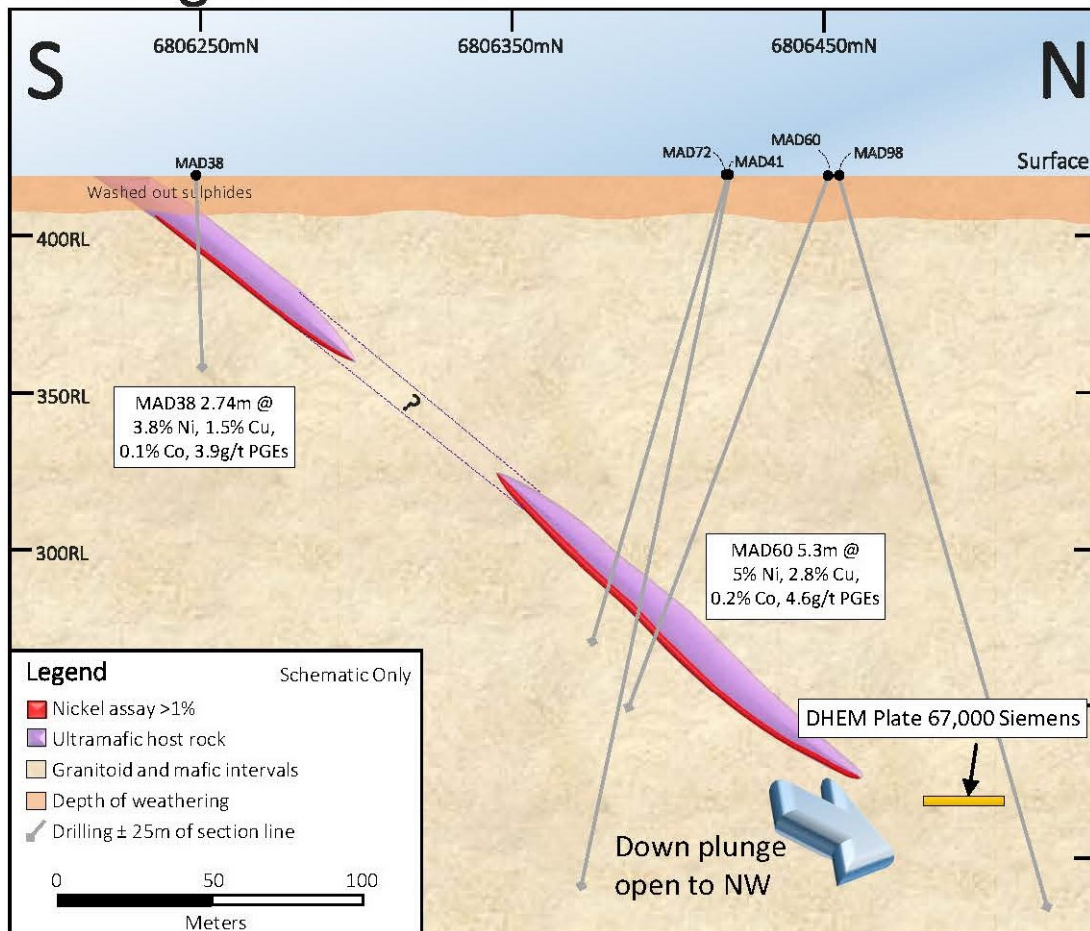
Figure 3 – Schematic cross section of the MAD60 line (facing west) at Investigators based on interpretation of drill hole data. The mineralised ultramafic dips to the north-west with potential for a down plunge extension, where the new DHEM conductor is located.
