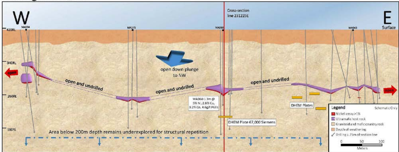
Figure 2 – Schematic long section of the Investigators Prospect (facing north) based on interpretation from drill hole data. Drill holes shown near the DHEM Plate 67,000 Siemens are to the south of the Plate and have not intersected the conductor.
