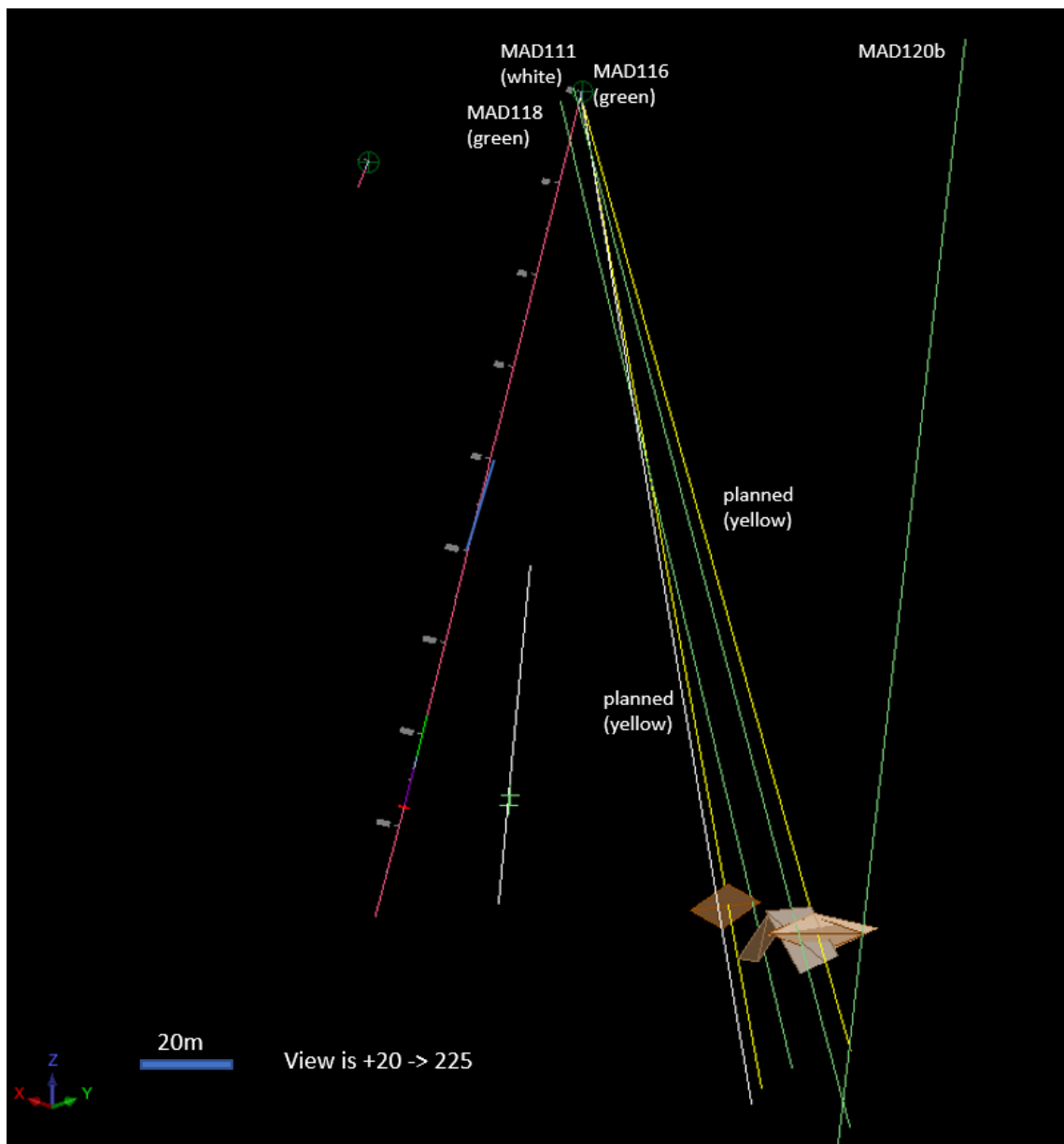
Figure 2 - Oblique view, looking up (+20 degrees) towards 225° +/-25m showing new DHEM plates. Planned drill holes are in yellow. Other drill holes shown (green and white) did not intersect the target plates (brown).
