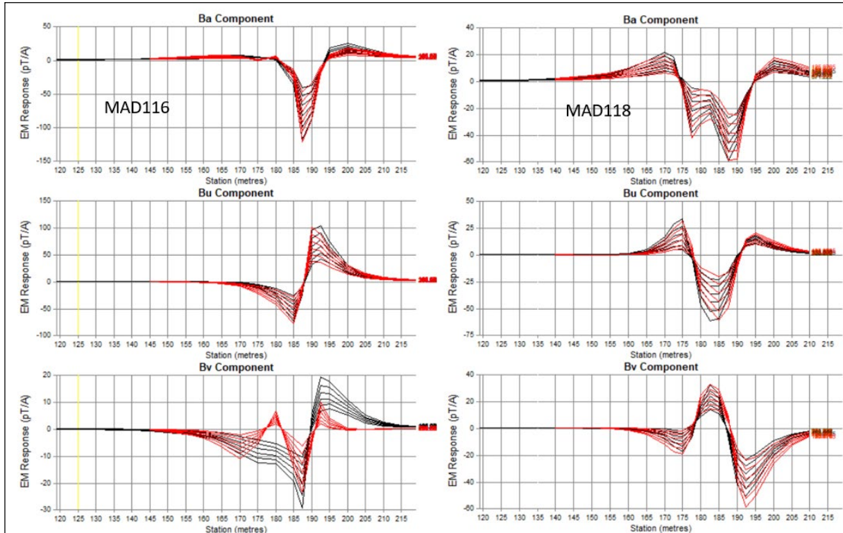
Figure 1 - MAD116 and MAD118 DHEM late time profiles of CH34 to CH39 (125ms to 371ms). Red profiles are modelled responses and black profiles are observed data. The sharp negative to positive cross-overs on the radial component (Bu, Bv) suggest a strong and proximal off-hole conductor.
