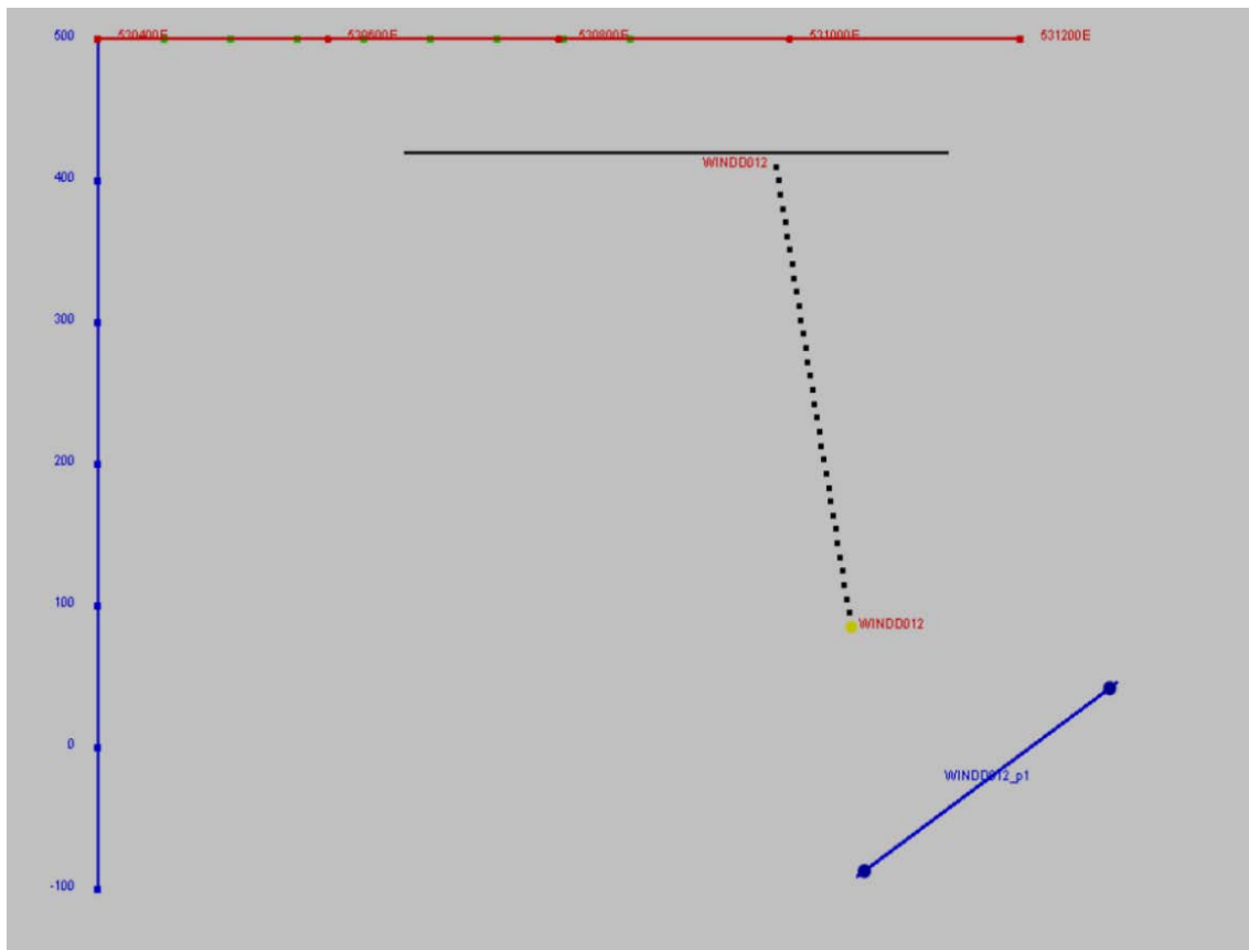
Figure 2 – section view looking north-west shows the new EM conductor below WINDD012.
