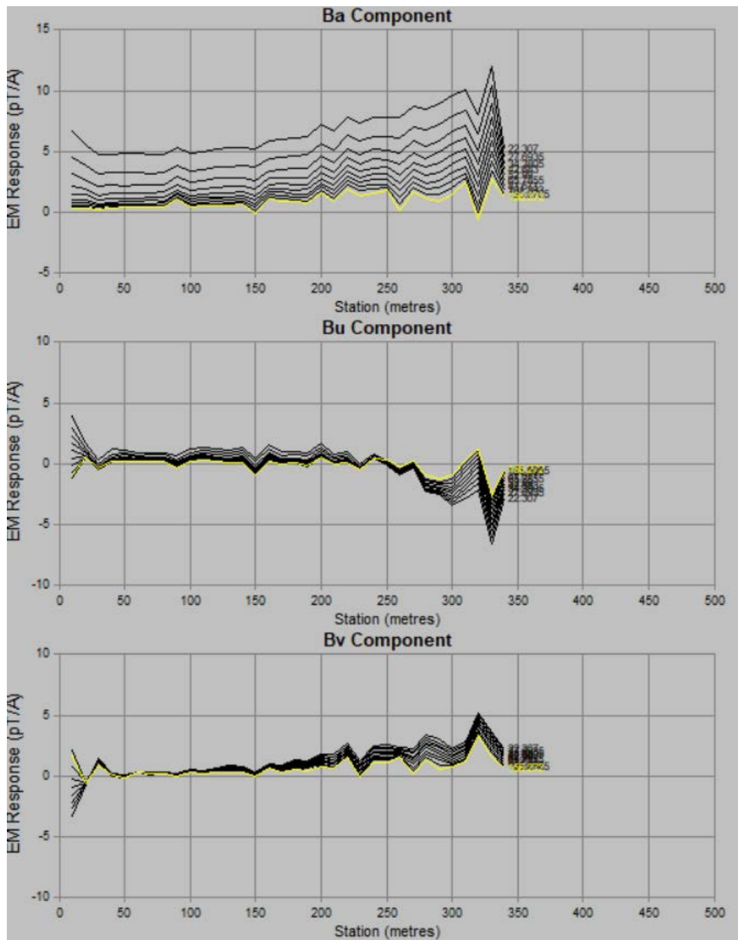
Figure 1 – DHEM survey data for WINDD012 in the late time linear profiles (22ms to 156ms) shows an increasing positive EM anomaly.
