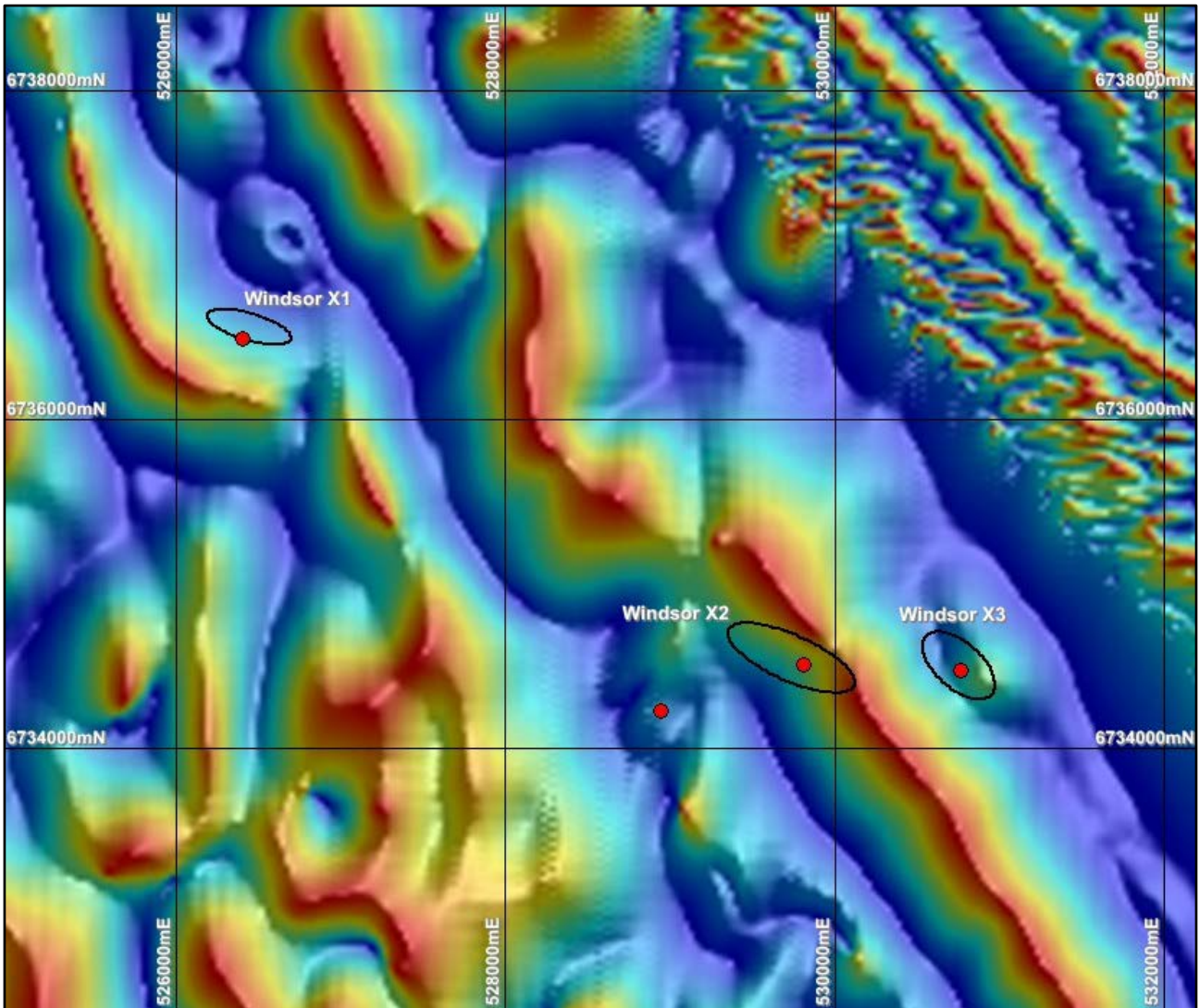
Figure 2 – map of the Windsor prospect (against RTP tilt mag data) showing the favourable location of Windsor X3 and the other EM conductors being tested. Planned drill holes are depicted by red dots. Windsor X3 is favourably located; it is co-incident with a magnetic feature as well as being on the edge of a gravity feature
