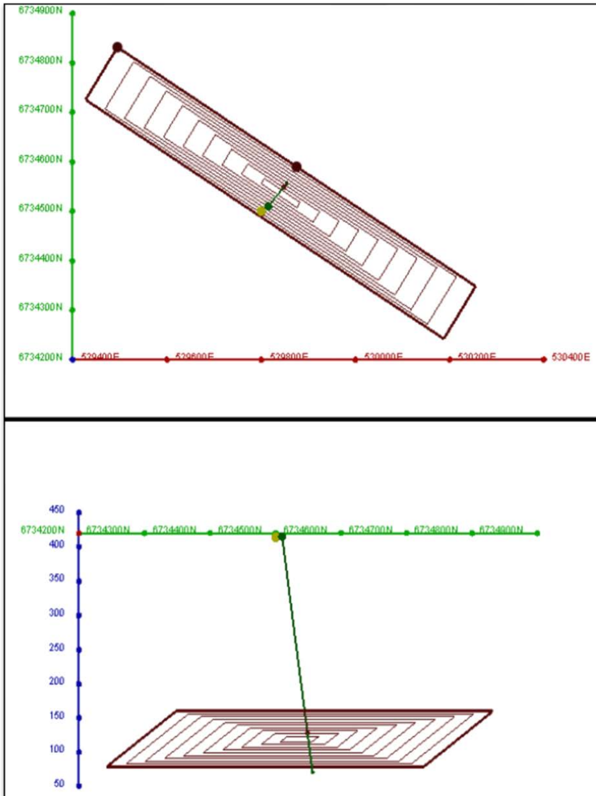
Figure 1 – modelled EM plate for Windsor X3 with planned drill hole WINDD012 (ELProp_02). Top panel: plan view of the EM plate and planned drill hole; Bottom panel: cross section looking west showing the flat lying EM plate and the planned drill hole trace.
