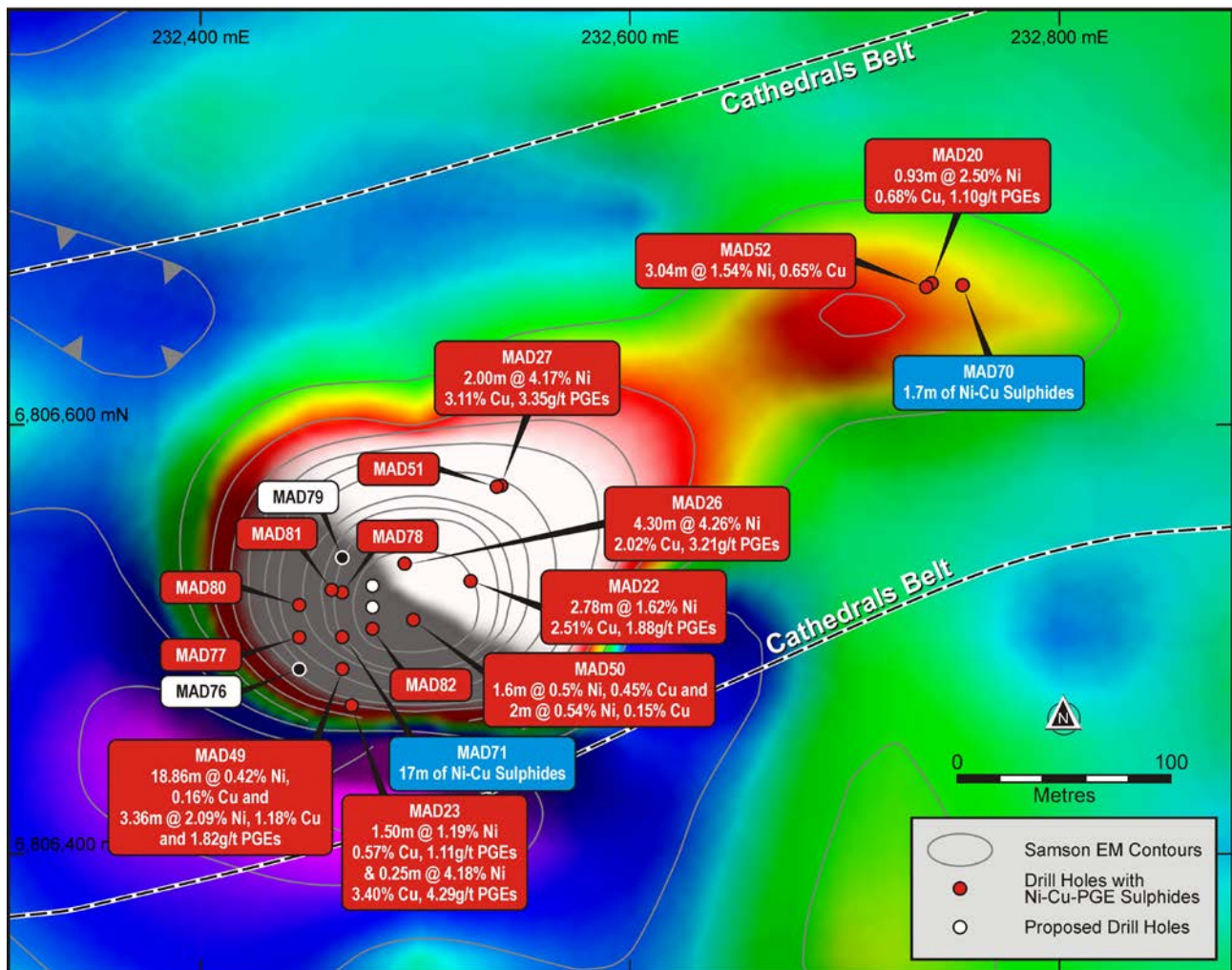
Figure 1 – a plan view of the Stricklands Prospect with drill hole collar locations over the large SAMSON total field EM anomaly (white/red colours). The SAMSON EM image is shown in Channel 18 (44ms). The contours shown are 0.05pT/A which highlight the stronger electromagnetic field over the Stricklands Prospect.
