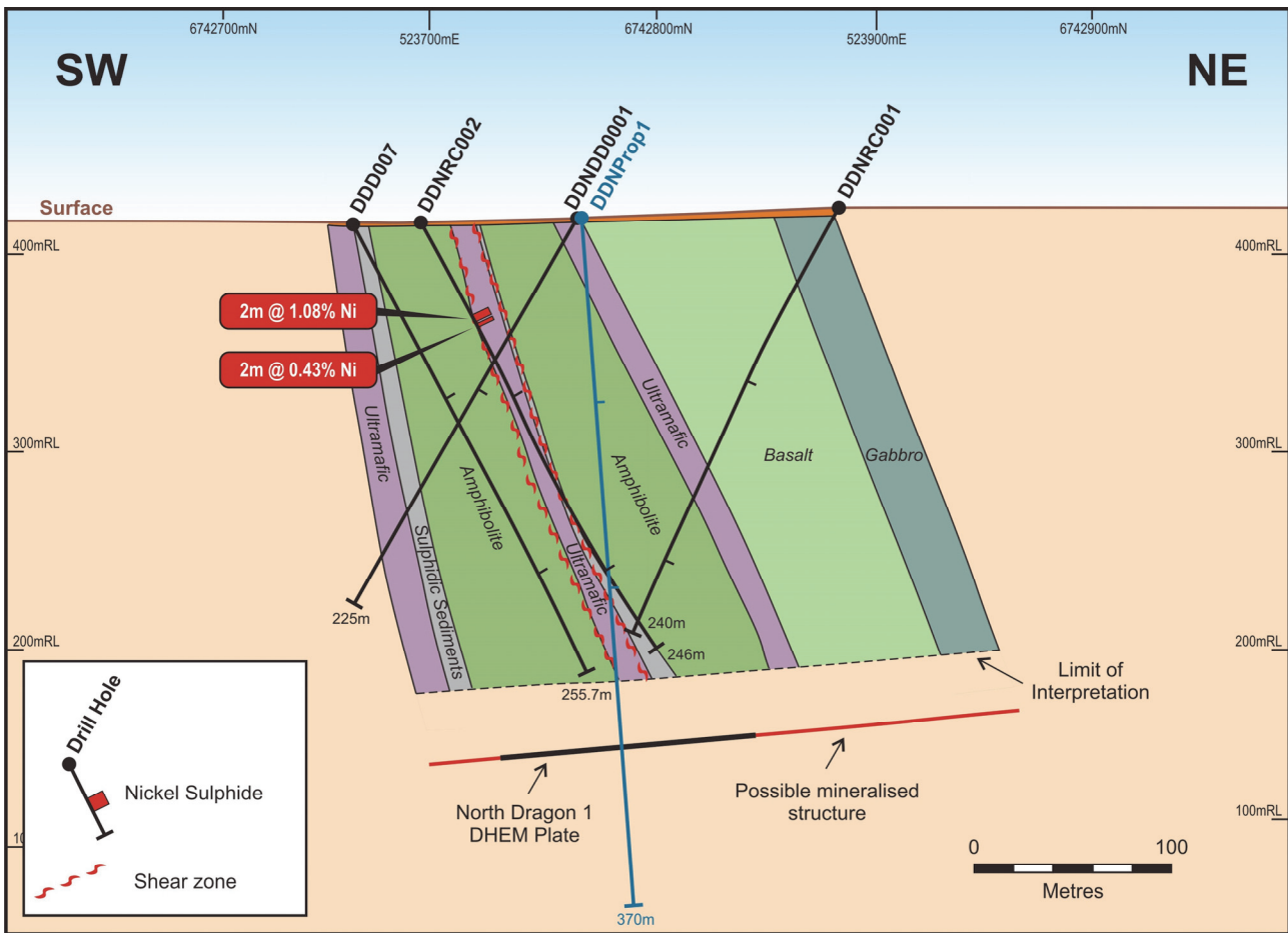
Figure 1 - Interpreted geology of the 'DDNRC002 cross section' at Desert Dragon North. Planned drill hole DDNProp1 is collared on section and will test the 'North Dragon 1' DHEM conductor 100m north of the section.
