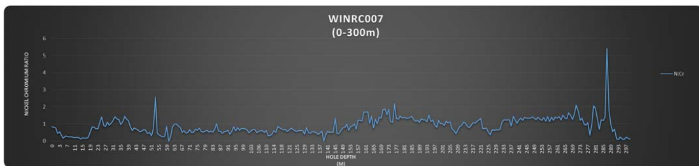
Figure 1 – XRF geochemical profile of WINRC007 showing the high Ni:Cr ratio
