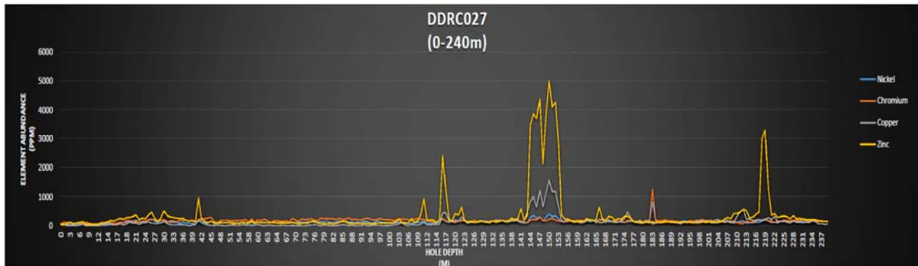
Figure 1- XRF profile of zinc and copper in DDRC027 showing mineralised interval
