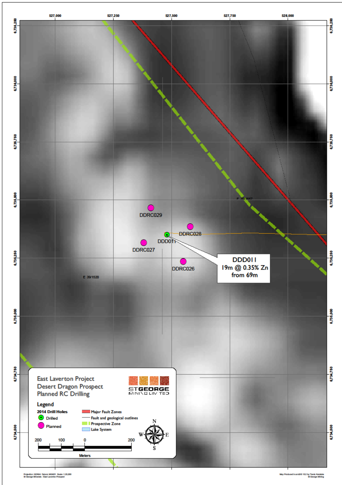
Figure 2 – the VMS prospect at Desert Dragon over 1VD magnetics. DDD011 and the planned drill holes are highlighted.
