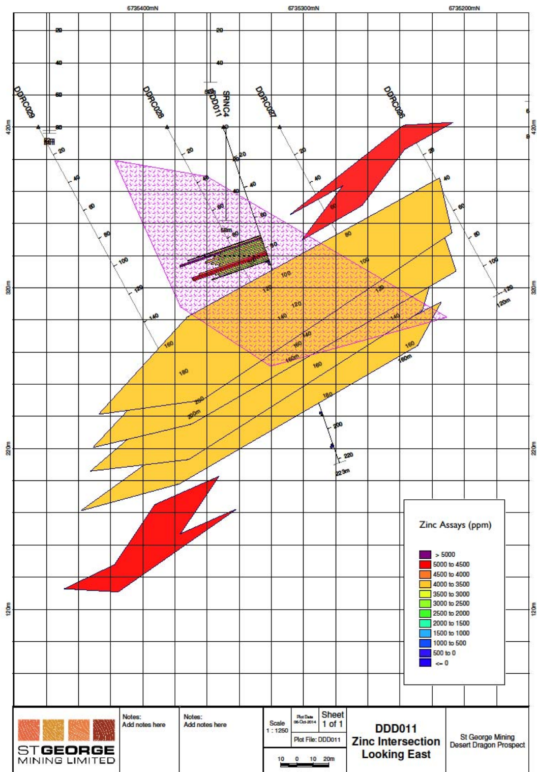
Figure 1 – A cross section of DDD011 highlighting the mineralised interval between 69m and 88m. The large yellow planes represent sedimentary units encountered. Planned holes DDRC026 to DDRC029 will test for an extension of the mineralised interval which is open along strike.
