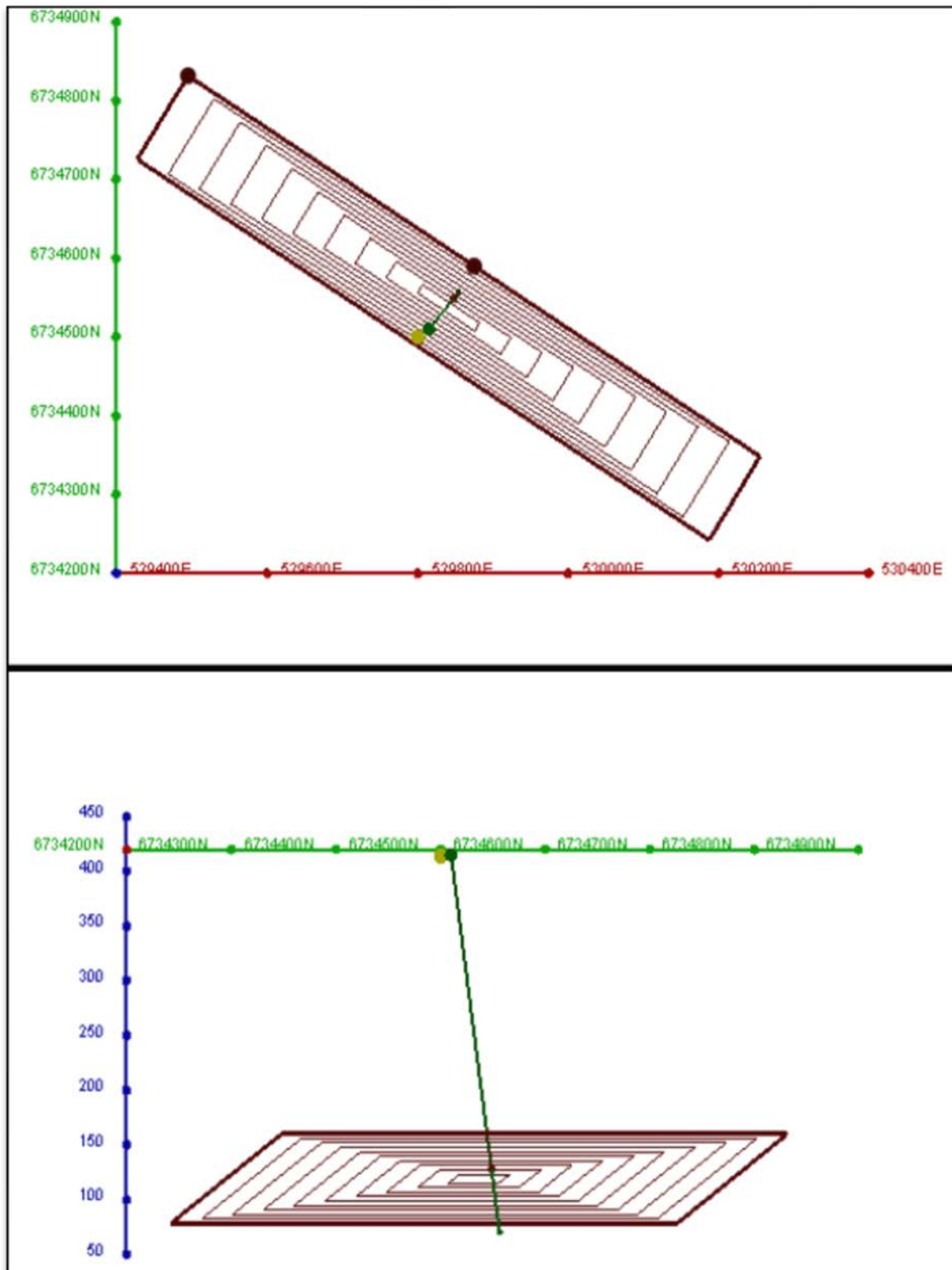
Figure 3 – modelled EM plate for Windsor X3 with planned drill hole ELProp_02. Top panel: plan view of the EM plate and planned drill hole; Bottom panel: cross section looking west showing the flat lying EM plate and the planned drill hole trace.
