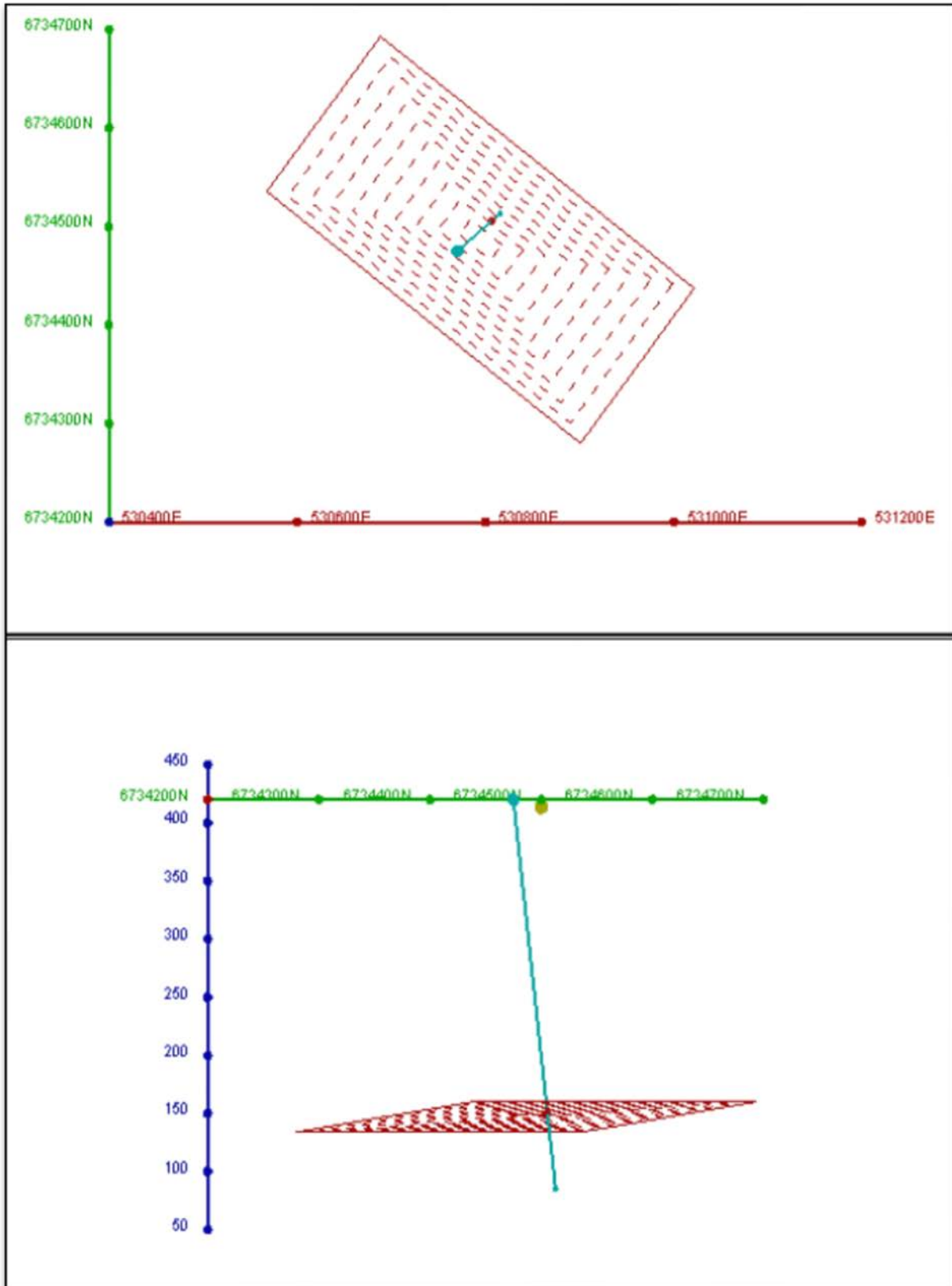
Figure 2 – modelled EM plate for Windsor X2 with planned drill hole ELProp_01. Top panel: plan view of the EM plate and planned drill hole; Bottom panel: cross section looking west showing the flat lying EM plate and the planned drill hole trace.
