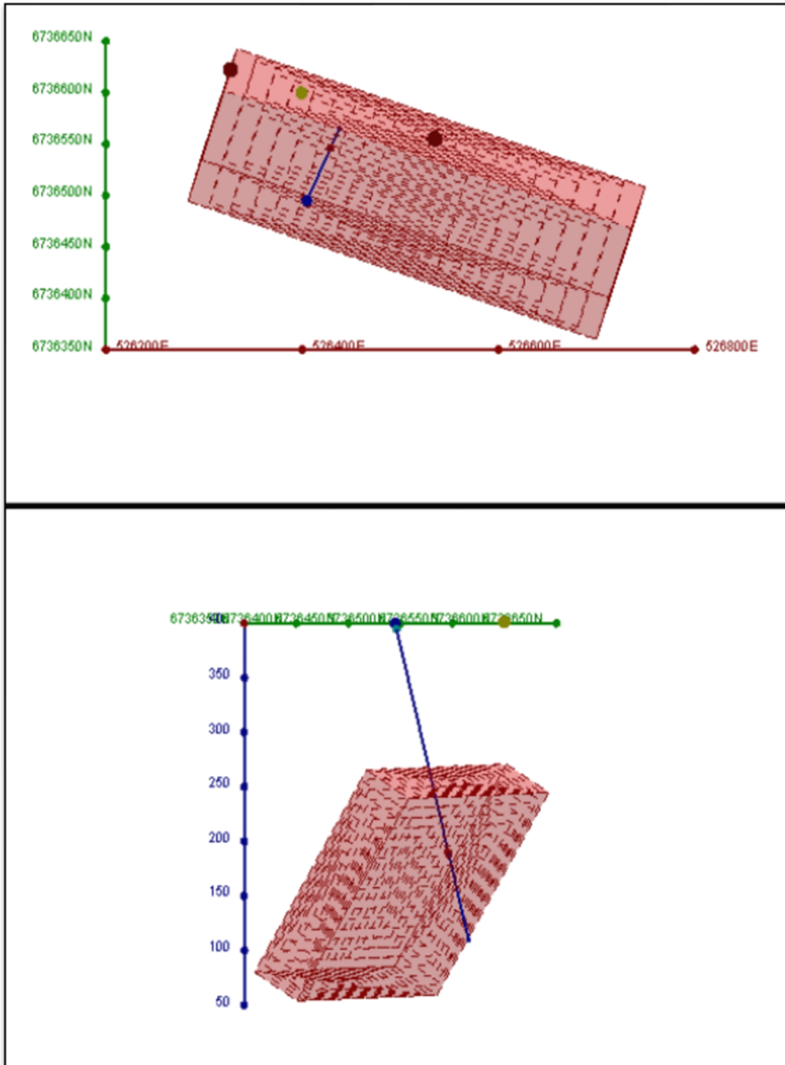
Figure 4 – modelled EM plate for Windsor X1 with planned drill hole ELProp_03. Top panel: plan view of the EM plate and planned drill hole; Bottom panel: cross section looking west showing the EM plate with a 60 degree dip and the planned drill hole trace.
