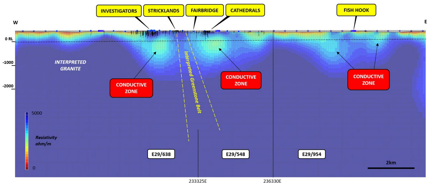
Figure 1 – long section (east-west, looking north) of the Cathedrals Belt with MT/AMT 3D inversion modelling of the survey data showing large conductive zones below the current extent of drilling.
