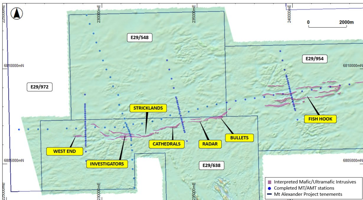
Figure 2 - map of the Cathedrals Belt showing key prospects and MT/AMT survey stations overlaying interpreted geology and magnetics (TMI RTP 1VD).
