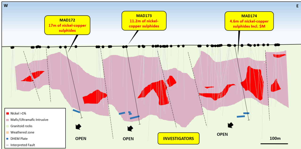
Figure 3 – schematic long section (+/-50m, looking north) of Investigators showing drill hole traces and location of new EM conductors down-plunge of known mineralisation. The location of MAD172, MAD173 and MAD174 and the EM plates that the holes targeted are highlighted.
