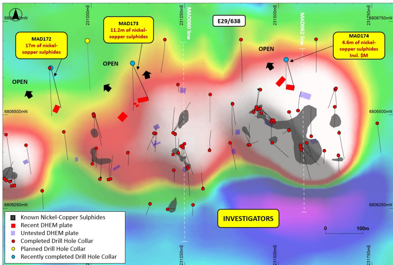
Figure 2 – plan view map of the Investigators Prospect (set against SAMSON CH18 data) highlighting the drilling to date, including MAD173 and MAD174, and the large number of untested EM plates. Mineralisation is open to the north and down-dip.
