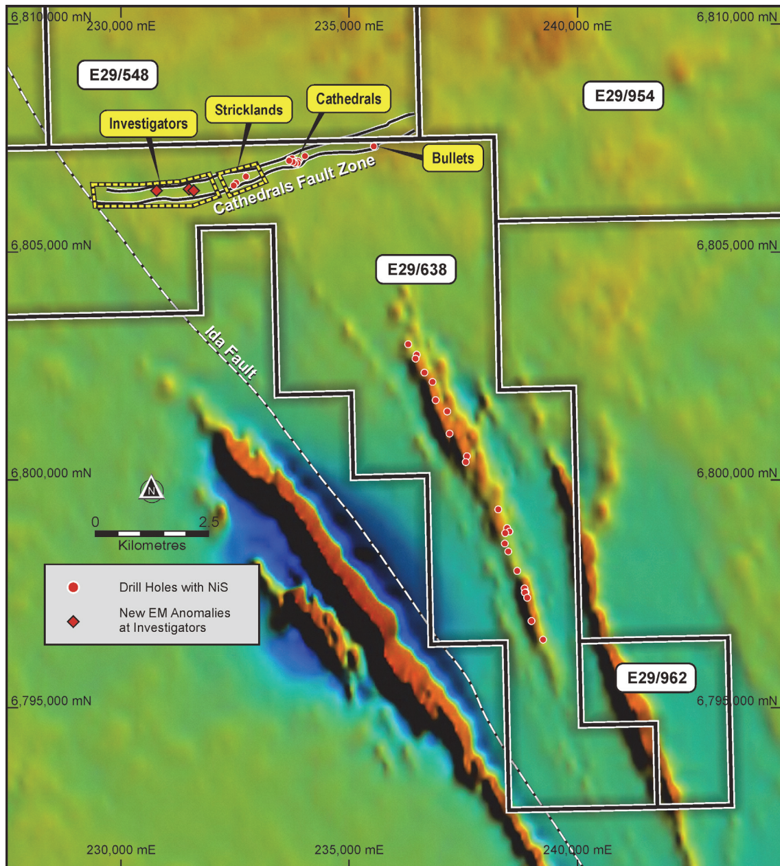
Figure 1 – a plan view of the Mt Alexander Project area over RTP magnetics. The new EM conductors at Investigators are within the same east-northeast structural corridor where high grade nickel-copper sulphides have been discovered at the Cathedrals and Stricklands Prospects.
