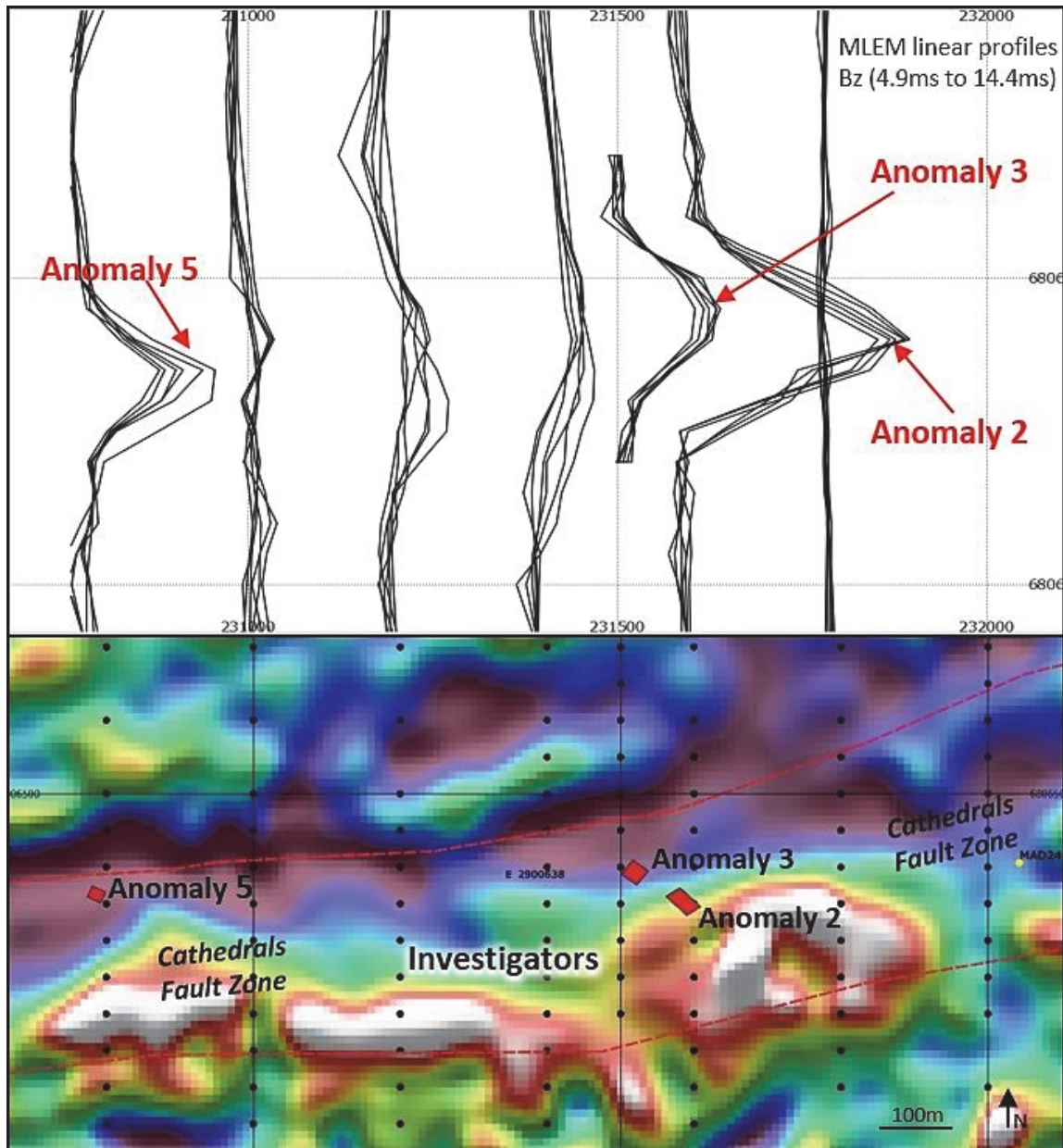
Figure 2 – the Investigators Prospect (against TMI 1VD magnetic data) showing the location of the three EM conductors as well as the survey stations from the MLEM survey. The EM responses from the survey highlight the very high conductivity of Anomaly 2.
