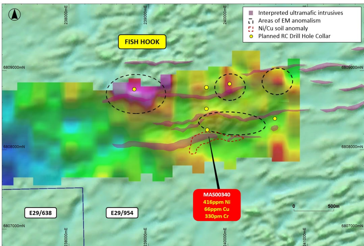
Figure 1 – map of the Fish Hook Prospect showing planned drill hole collars as well as the location of the large nickel soil anomaly and SQUID MLEM (CH28Z) anomalism against magnetic (RTP 1VD) data.
