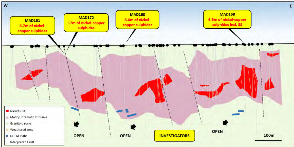
Figure 4 – schematic long section (+/-50m, looking north) of Investigators showing drill hole traces and location of new EM conductors down-plunge of known mineralisation. The location of MAD172 and the deeper EM plate that the hole targeted are highlighted.
