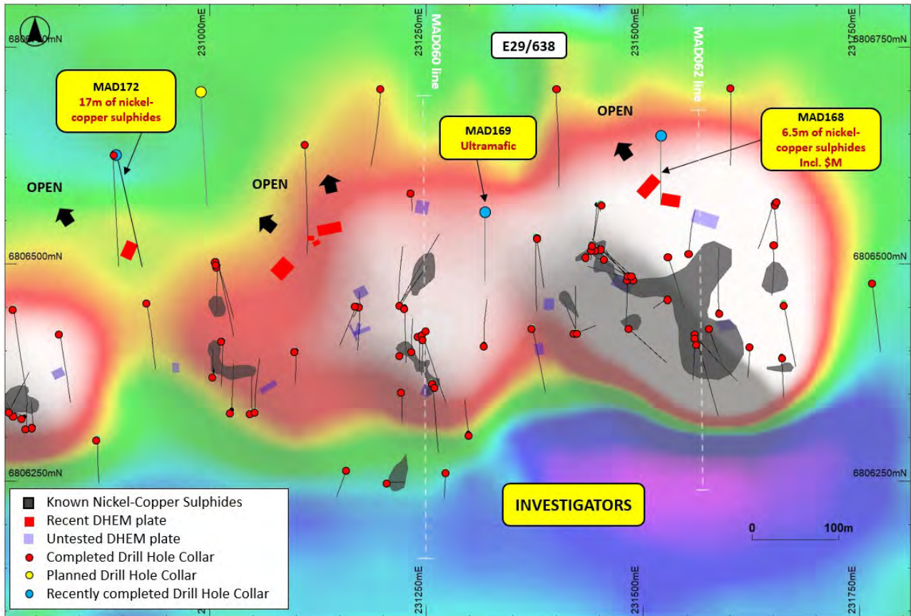
Figure 2 – plan view map of the Cathedrals Belt (set against SAM data) highlighting the location of MAD172 as well as the deeper drill holes recently completed at the Investigators Prospect and the large number of untested EM plates.
