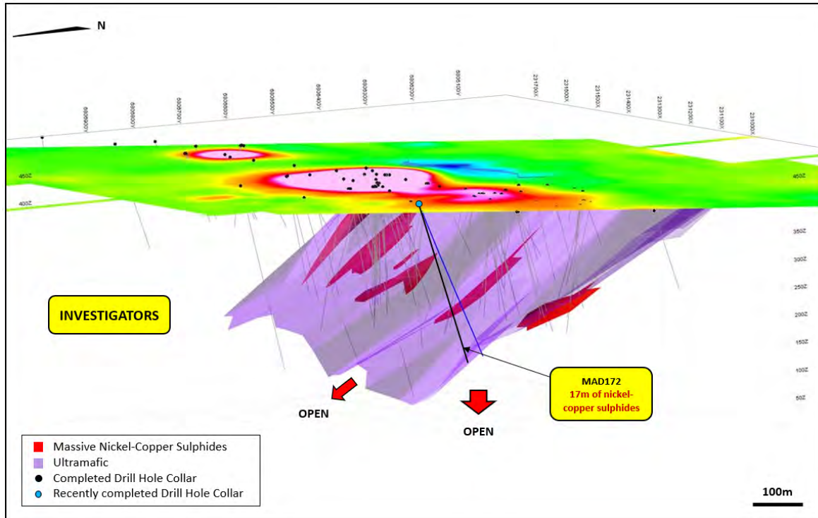
Figure 5 – 3D orthographic view (looking south-east) of the Investigators ultramafic showing drill holes and known massive nickel-copper sulphide mineralisation. The surface image is the SAMSON EM data and illustrates the large EM anomaly at Investigators. MAD172 has extended the down-plunge strike of nickel-copper sulphide mineralisation which remains open.
