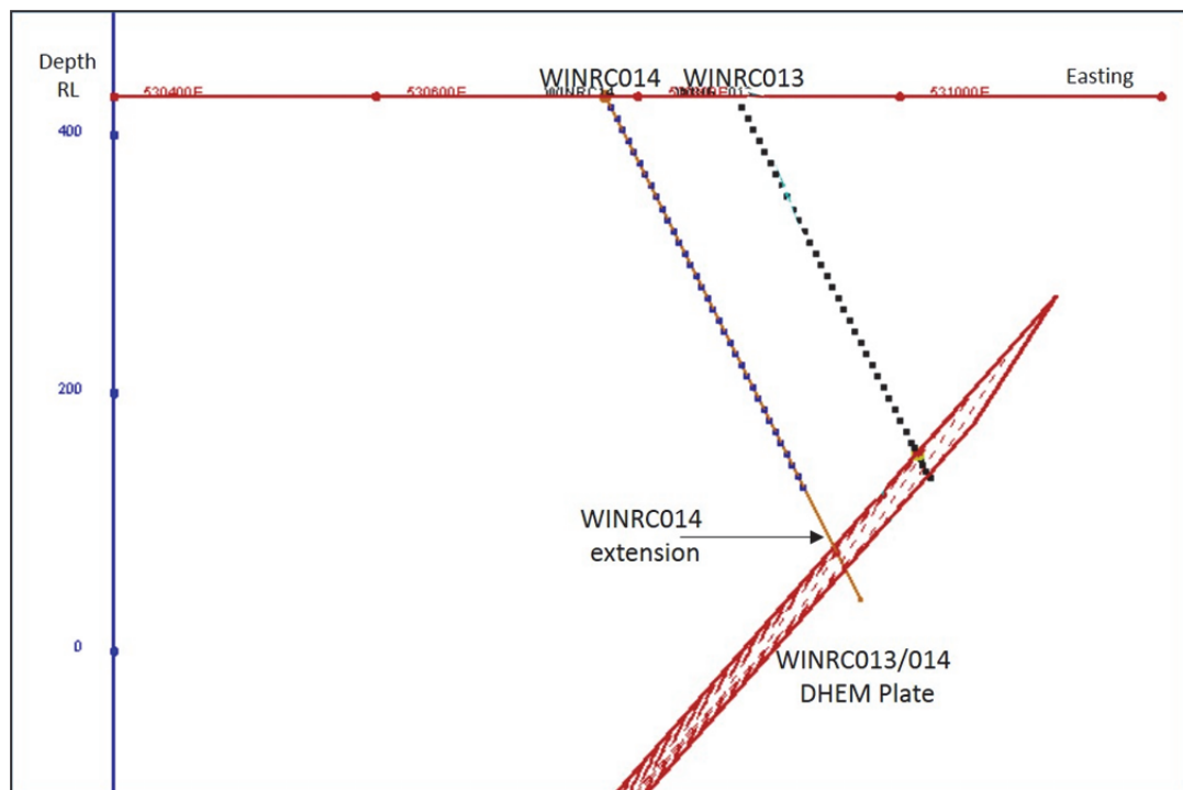
Figure 2 – the modelled DHEM plate for the off-hole conductor to be tested by the extension of WINRC014. WINRC013 did not intersect the conductor.
