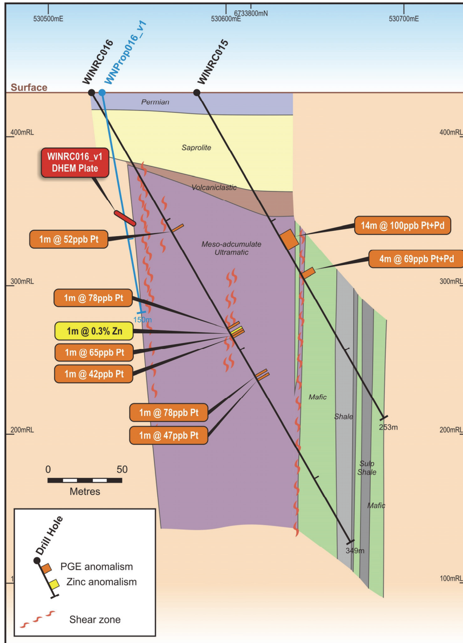
Figure 1 – Interpreted geological cross section of WINRC016 and WINRC015 (+/-50m), showing the prospective Windsor ultramafic with PGE intersections. The extremely conductive WINRC016_v1 plate is situated on the western contact of the Windsor ultramafic and will be tested by the planned hole shown
