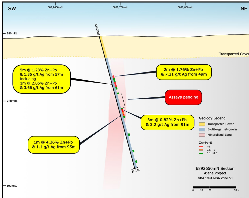
Figure 4: schematic cross-section of AJRC002 at the Perseverant Prospect.
