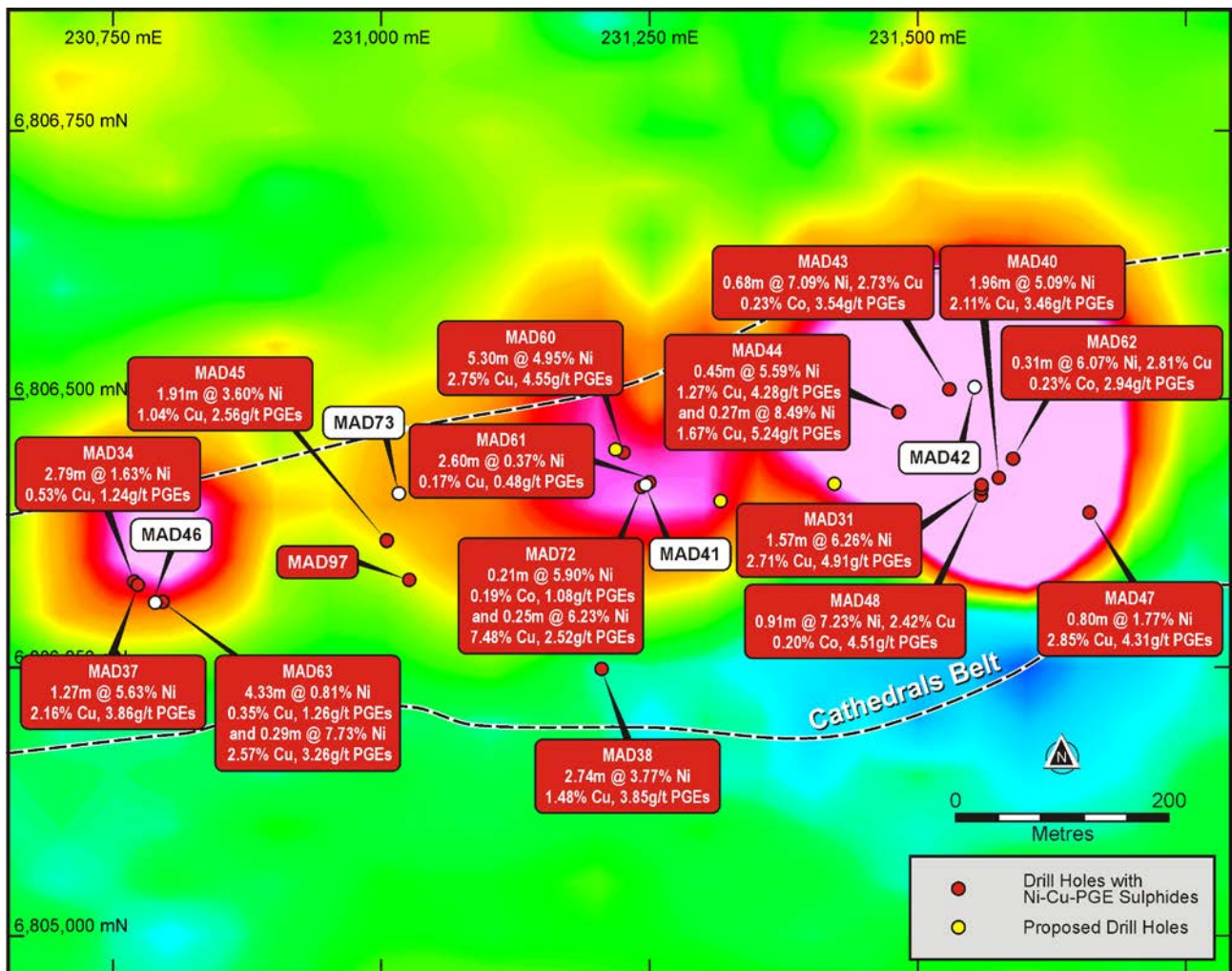
Figure 3 – plan view of Investigators Prospect with drill hole collar locations (completed and planned) over the large SAMSON total field EM anomalies (red/pink colours). SAMSON EM image is shown in Channel 18 (44ms).
