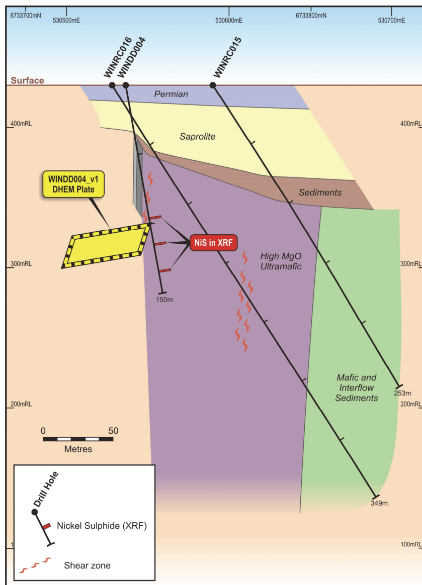
Figure 1 – Interpreted geological cross section of WINDD004, WINRC016 and WINRC015 (+/-50m) showing the location of the highly conductive WINDD004_v1 plate on the western contact of the Windsor ultramafic.
