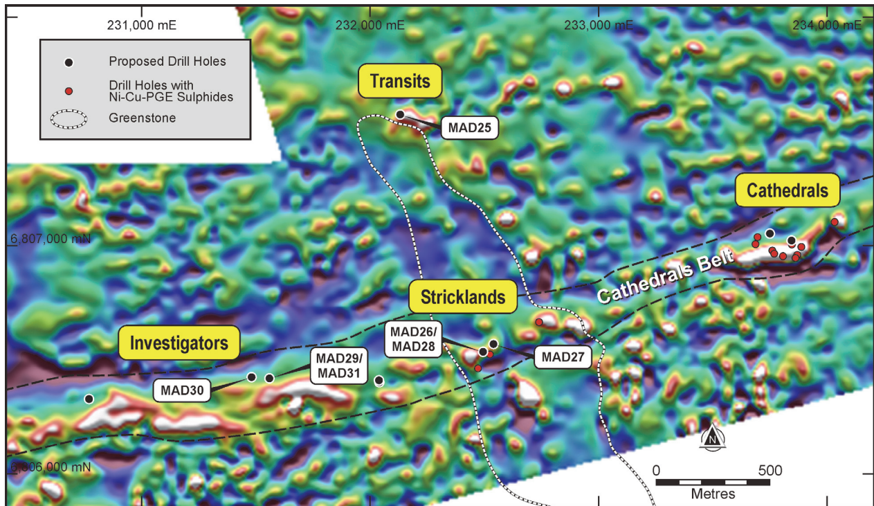
Figure 2 – a plan view of the Cathedrals Belt over TMI magnetics showing the drill hole collar locations in the current programme. MAD25-MAD30 are the drill holes completed to date.
