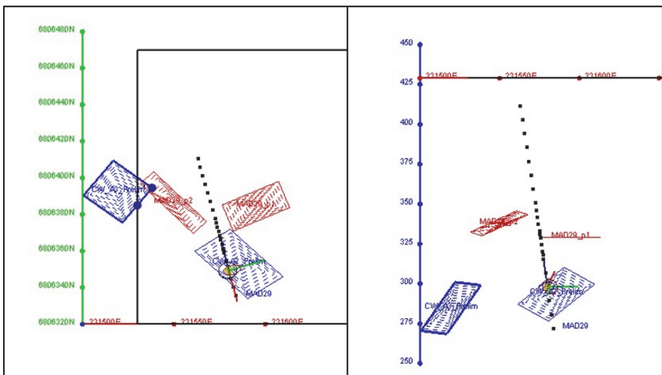
Figure 1 – the new DHEM plates (red) from the MAD29 DHEM survey and previous MLEM plates (blue) for Anomaly 2 and Anomaly 3 at Investigators. Image on the left shows the plan view and on the right is a cross section looking north. The MAD29 drill hole is in black.
