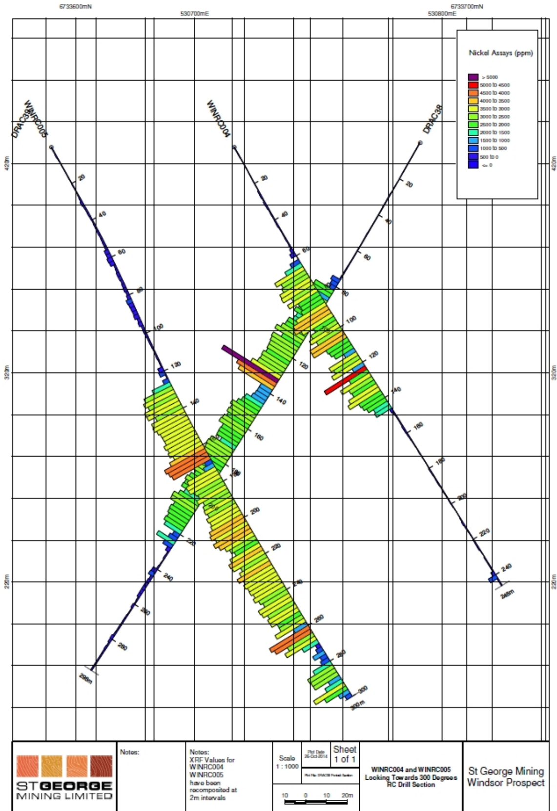
Figure 2 – A cross section of the drill holes at Windsor which highlights the unconstrained zone of nickel sulphides
