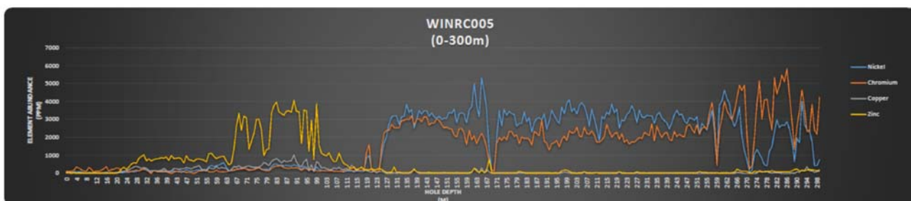
Figure 1 - XRF geochemical profile of WINRC005
