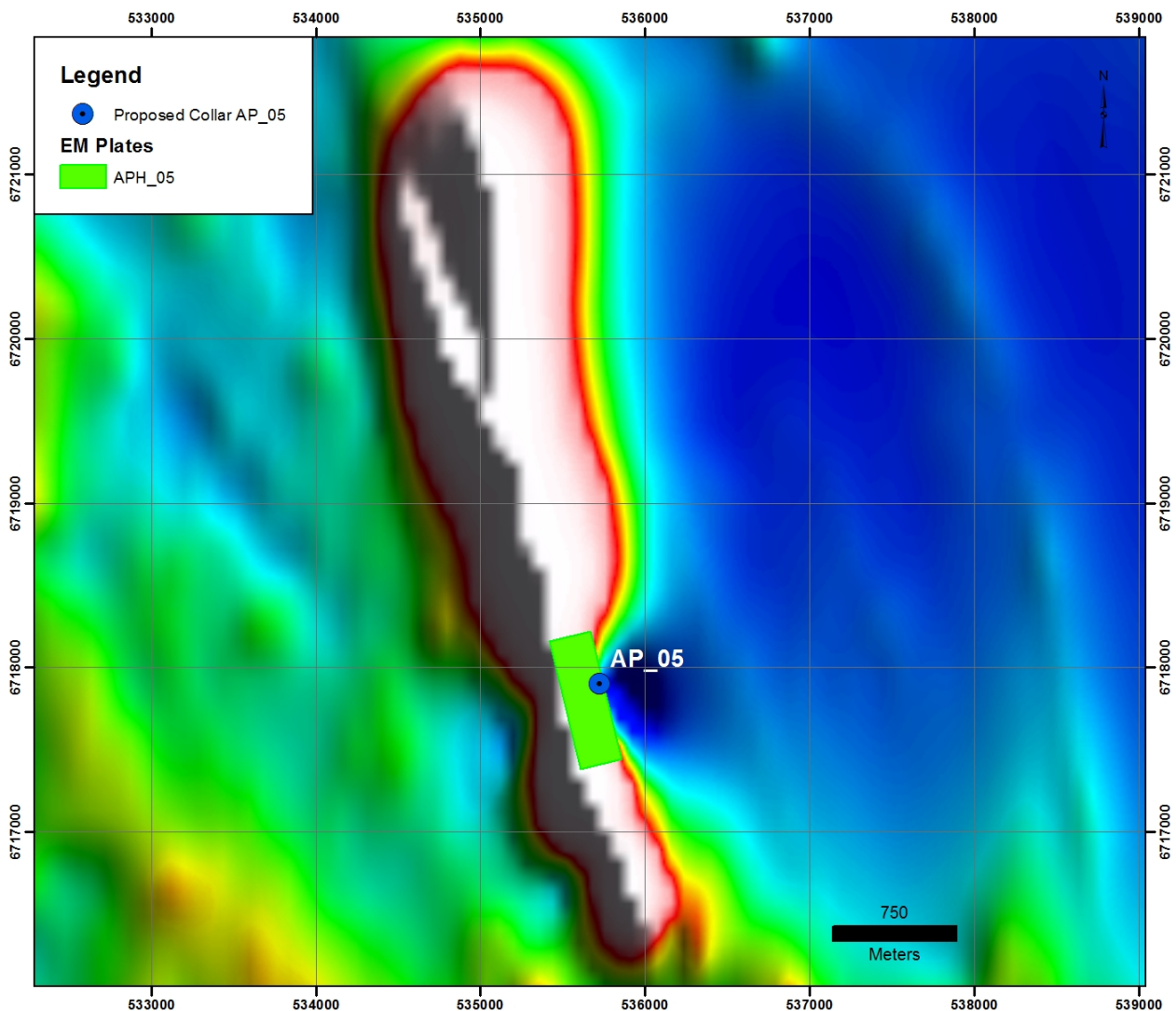
Figure 3 - Aphrodite 4, to be tested by drill hole AP_05, is situated in a pronounced indentation of the ultramafic body. This 'embayment' is a highly favourable site for massive nickel sulphides.
