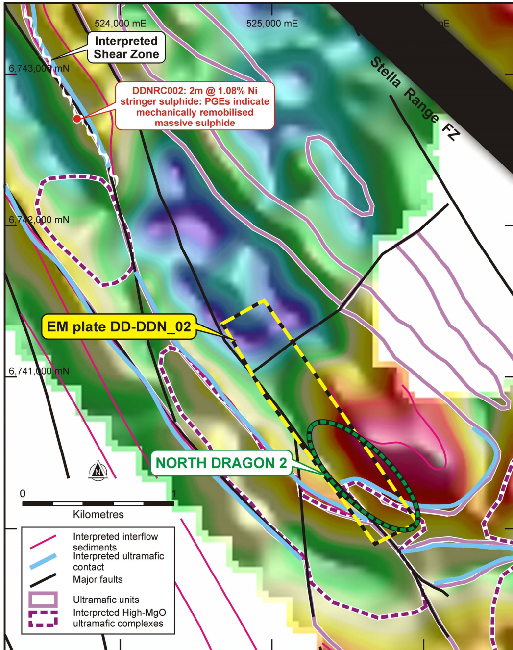
Figure 4 – Desert Dragon North against gravity data. North Dragon 2 is a strong late-time conductor that lies along the western margin of a strong gravity high, which is likely to represent sulphide-rich rocks
