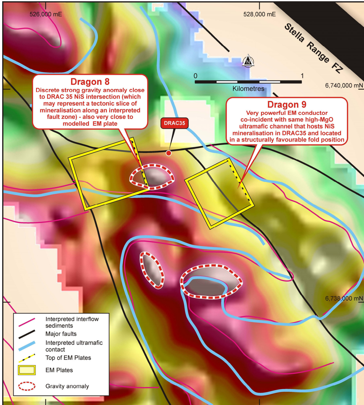
Figure 1 – a map of Desert Dragon Central against gravity data. The two EM conductors to be tested are located on the ultramafic contact of a high-MgO ultramafic complex - a high priority target zone for massive nickel sulphides. The location of the targets in the limb of a very prominent fold 'nose' in the Stella Range belt is also favourable for the structural concentration of massive nickel sulphides. Drill hole DRAC35 was completed at Desert Dragon Central by BHP Billiton Nickel West in 2012 and intersected 18m @ 0.40%Ni from 100m (including 4m @ 0.57%Ni from 100m).
