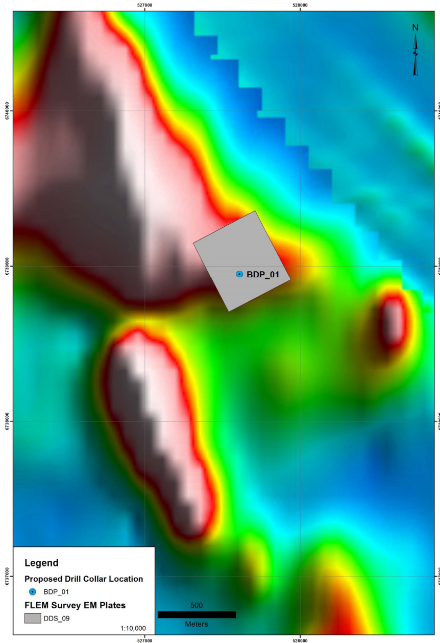
Figure 2 – a plan view of the EM plate for Dragon 9 and the planned hole BDP_01, against regional RTP magnetics data.
