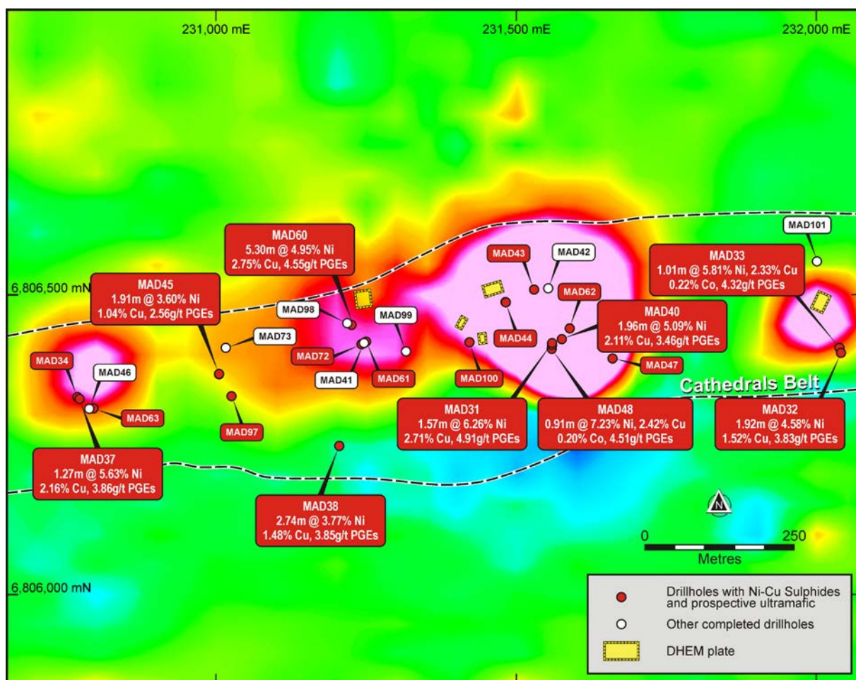
Figure 1 - plan view of Investigators Prospect with drill hole collar locations over the large SAMSON total field EM anomalies (red/pink colours). SAMSON EM image is shown in Channel 18 (44ms). The surface projection of the untested DHEM plates is also shown. Assays for completed drill holes are contained in Table 2 below.
