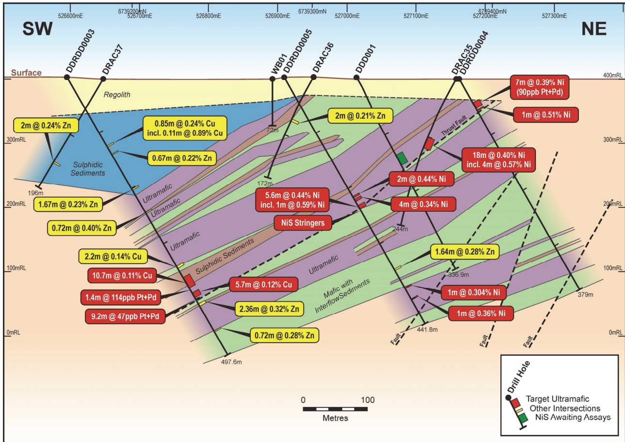
Figure 1 – Interpreted geological cross section from drilling at Desert Dragon Central. The multiple intersections of nickel sulphides and related anomalism are shown in red.
