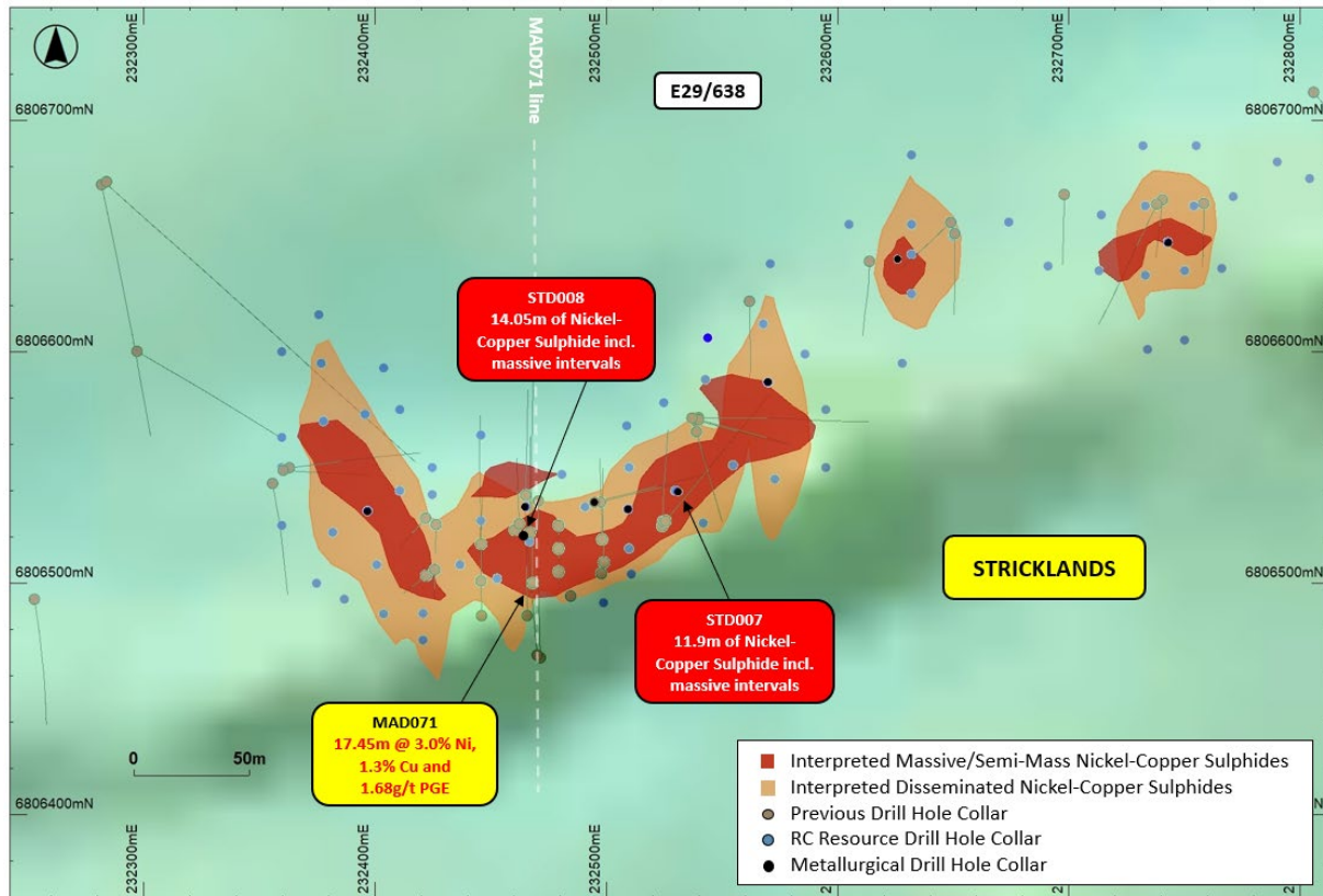
Figure 1 – schematic diagram of Stricklands (against TMI RTP 1VD magnetic data) showing the location of the RC and diamond drill holes completed as part of the resource development drill programme.
