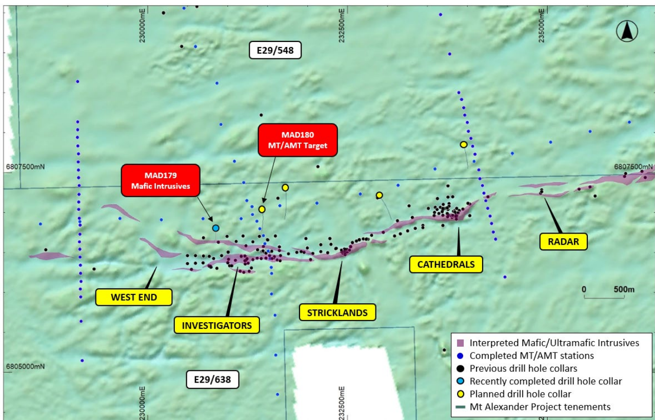
Figure 3 – Plan view of the Cathedrals Belt showing areas of completed and planned drilling, overlaying interpreted geology and magnetics (TMI RTP 1VD).
