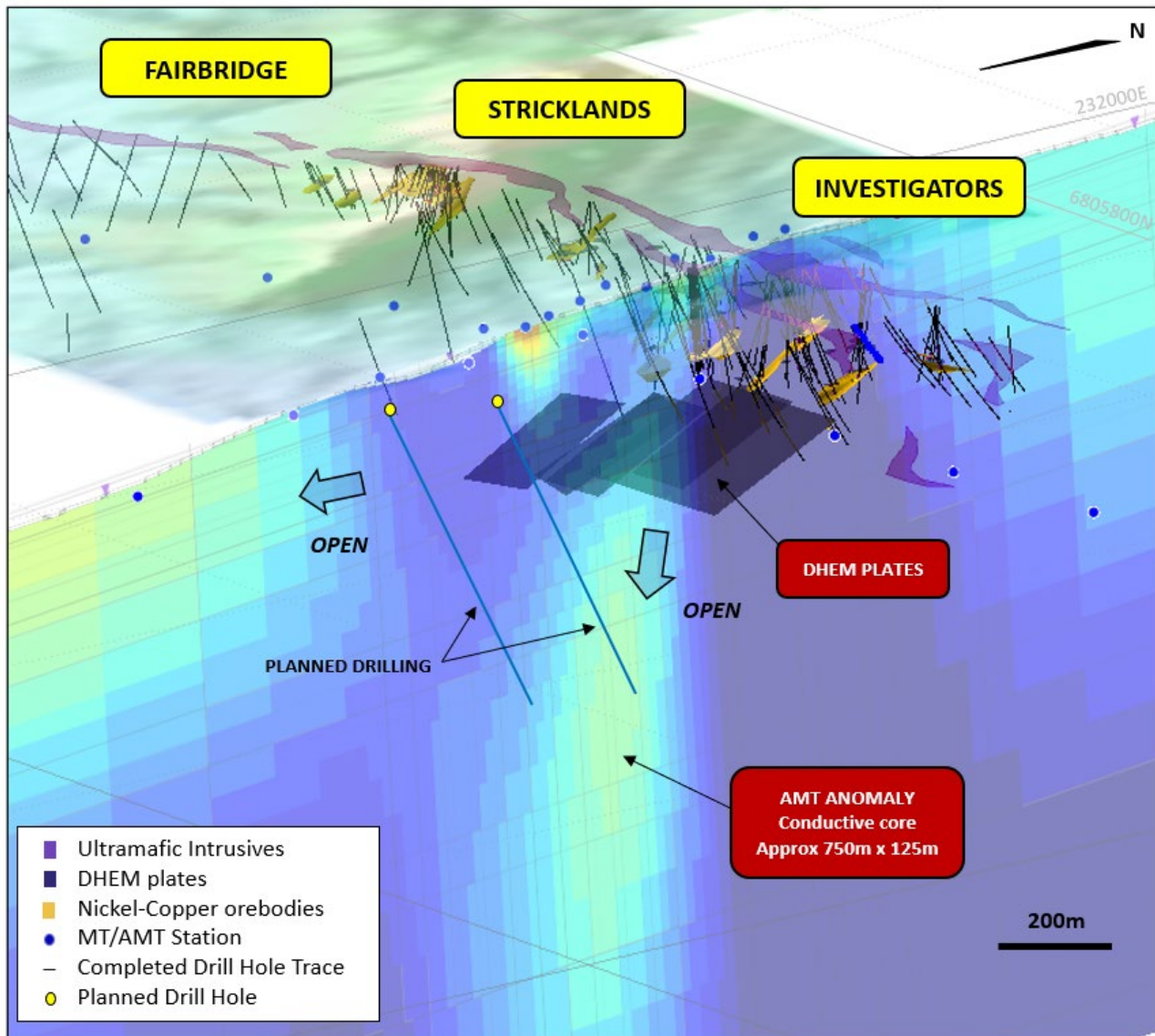
Figure 2 – oblique section (looking south-east) of Investigators showing a 2D section of the AMT data with the large AMT anomaly at depth and the planned holes to drill the target. The location of existing DHEM plates, past drilling and known shallow nickel-copper orebodies are shown, overlaying topographic DTM.
