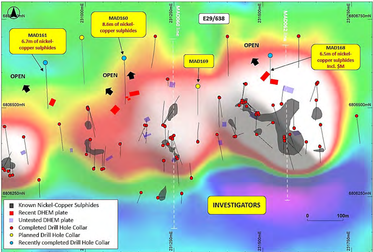
Figure 2 – plan view map of the Cathedrals Belt (set against SAM data) highlighting the deeper drill holes recently completed at the Investigators Prospect and the large number of untested EM plates.
