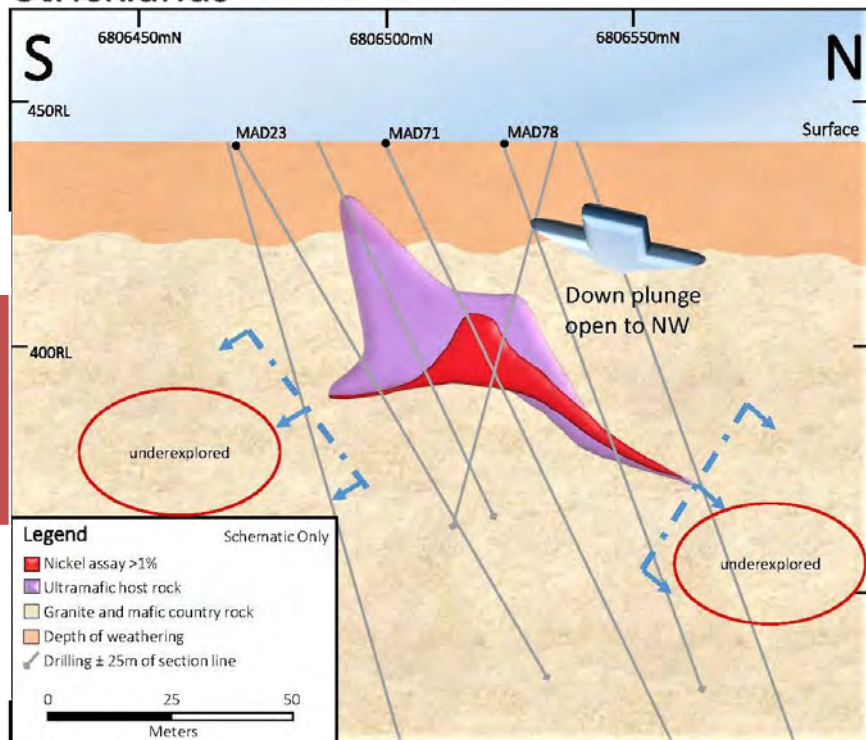
Above: Schematic cross section of the MAD71 line (facing west) at Stricklands based on drill hole data. The mineralised ultramafic dips to the north-west with potential for a down plunge extension.
