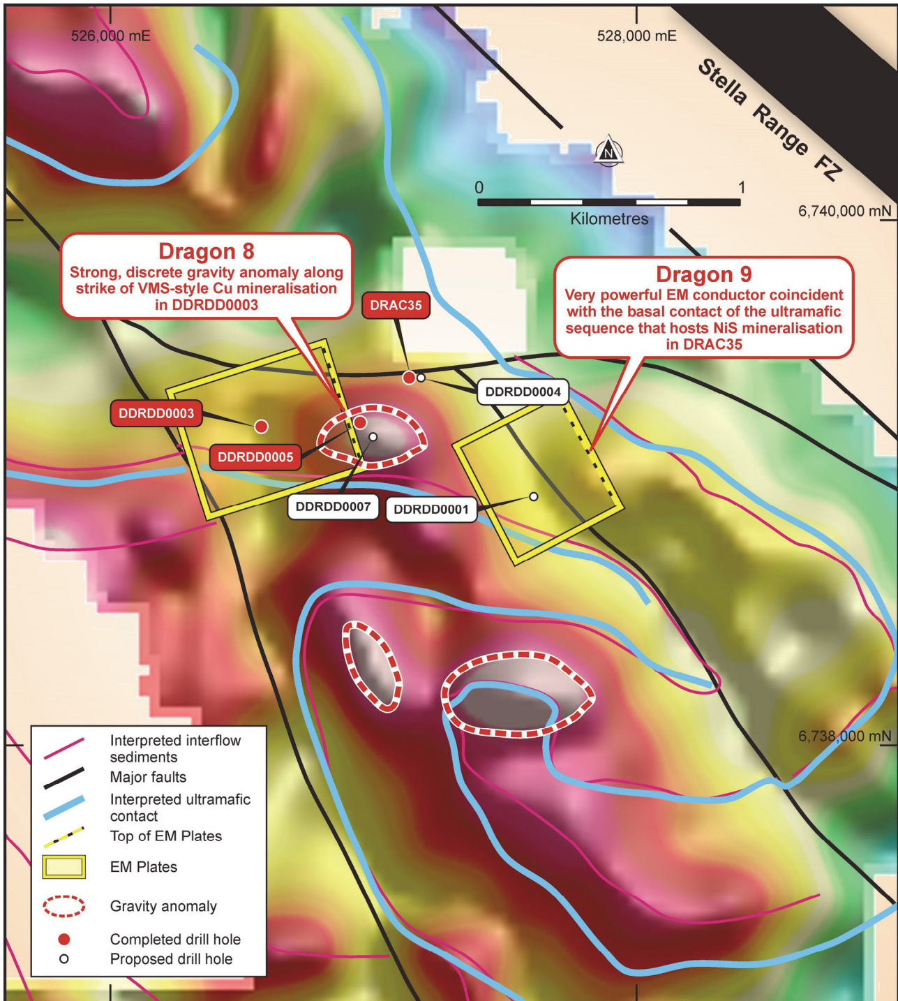
Figure 1 – a map of Desert Dragon Central against gravity data highlighting key targets. DDRDD0007 is being drilled into the centre of the Dragon 8 gravity anomaly that was only partially intersected by DDRDD0003 and DDRDD0005, both of which encountered zones of base metal mineralisation. The centre of the gravity anomaly may represent a larger accumulation of high grade mineralisation.
