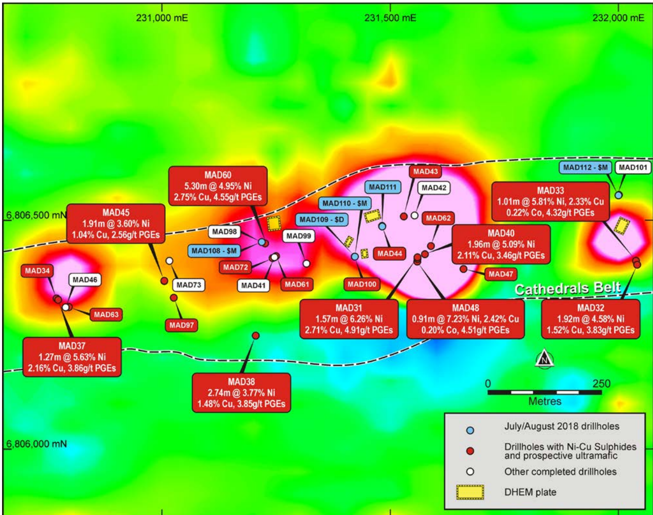
Figure 1 - plan view of the Investigators Prospect with drill hole collar locations over the large SAMSON total field EM anomalies (red/pink colours). SAMSON EM image is shown in Channel 18 (44ms). Drill holes from the current drill programme are shown, together with the surface projection of the DHEM plates being tested.
