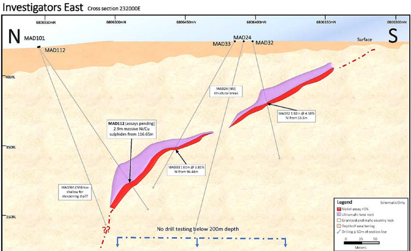
Figure 2 – schematic cross section of the MAD112 line (facing east) at Investigators based on interpretation of drill hole data. The mineralised ultramafic dips to the north with MAD112 suggesting potential for further mineralisation down plunge.
