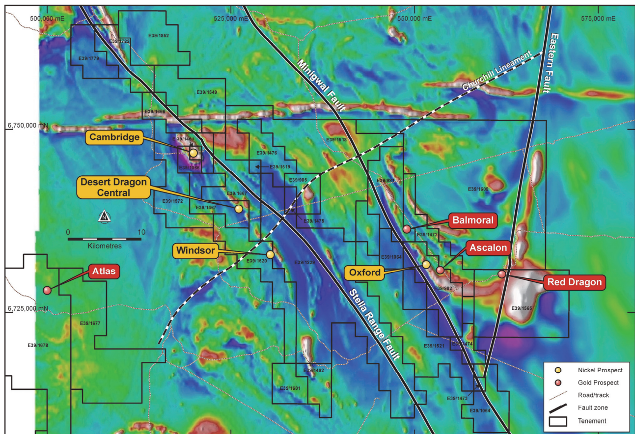
Figure 1 – St George’s tenements at East Laverton (against TMI magnetics) with the nickel sulphide and gold targets to be drilled in the RC drill programme currently underway.
