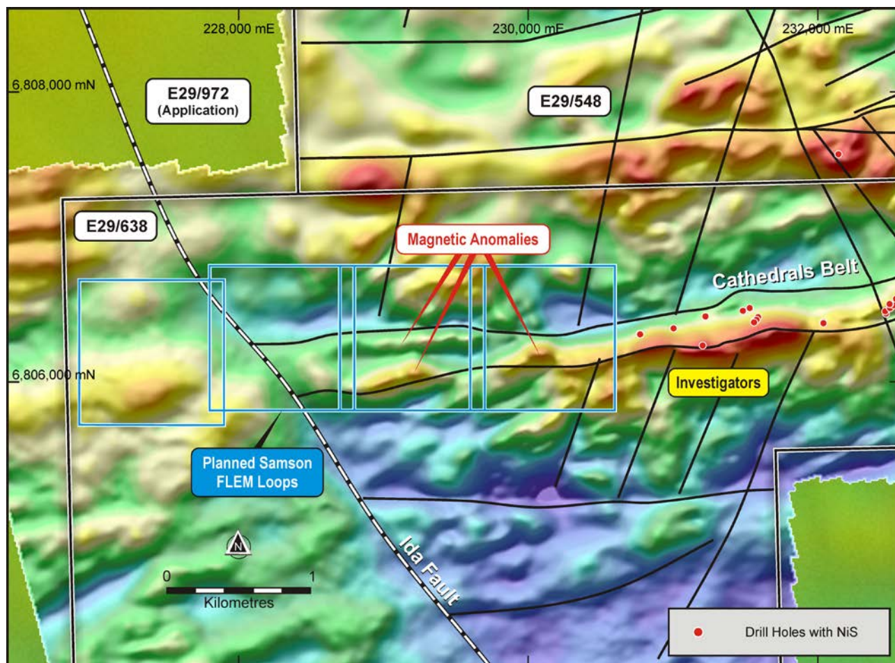
Figure 2 – a map of the western extension of the Cathedrals Belt (over TMI magnetics) with planned SAMSON EM loops shown. The SAMSON survey will cover the intersection of the Cathedrals Belt and the Ida Fault, which is west of the successful drilling at the Investigators Prospect.
