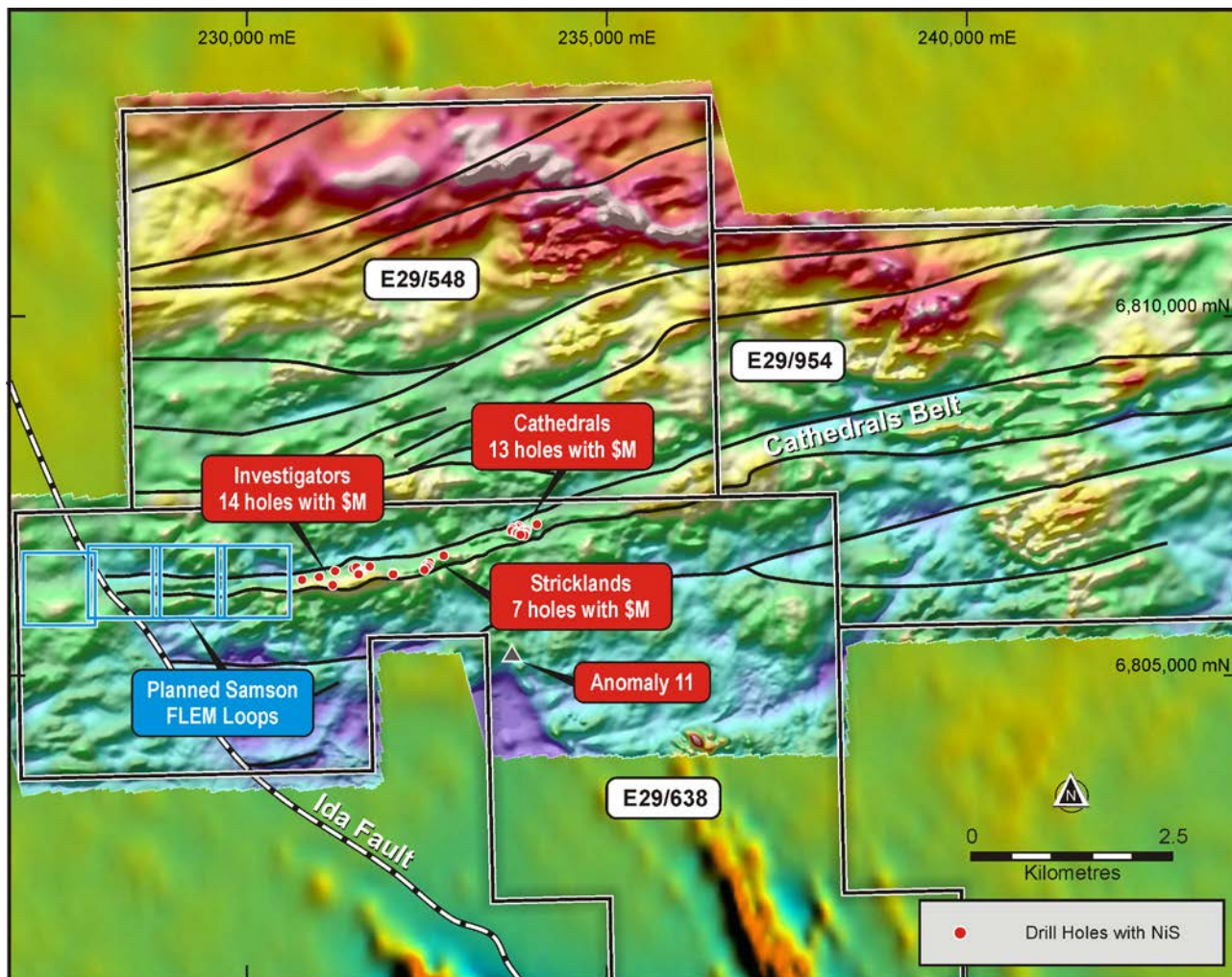
Figure 1 – a map of the Cathedrals Belt (against high resolution Total Magnetic Intensity) showing the location of the SAMSON EM loops planned for the area west of Investigators and across the Ida Fault. Intersections of massive nickel-copper-cobalt-PGE sulphides (“$M”) at the Investigators, Stricklands and Cathedrals Prospects are also highlighted.
