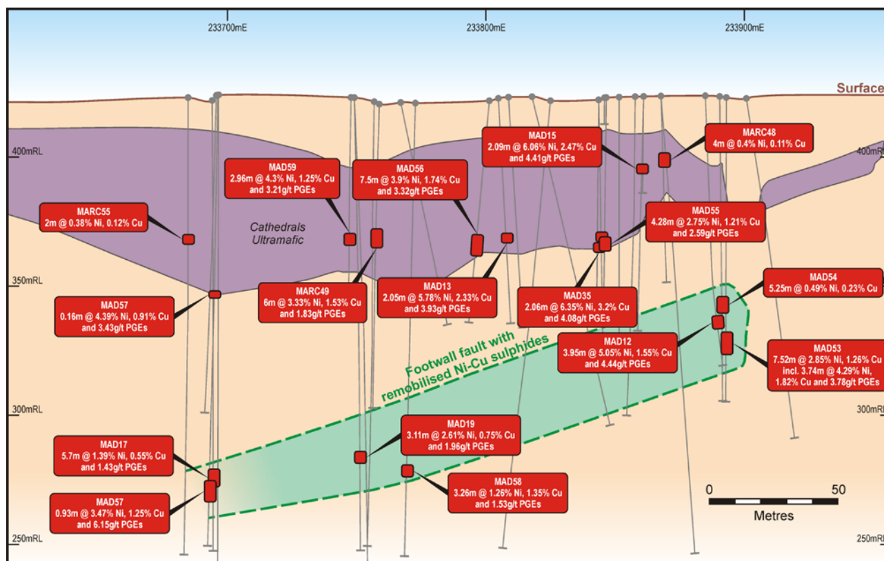
Figure 4 - a long section of the Cathedrals Prospect (looking north) showing significant intersections from both recent and historic drill holes. Further drilling of the Cathedrals ultramafic and footwall fault will test for an extension of mineralisation.
