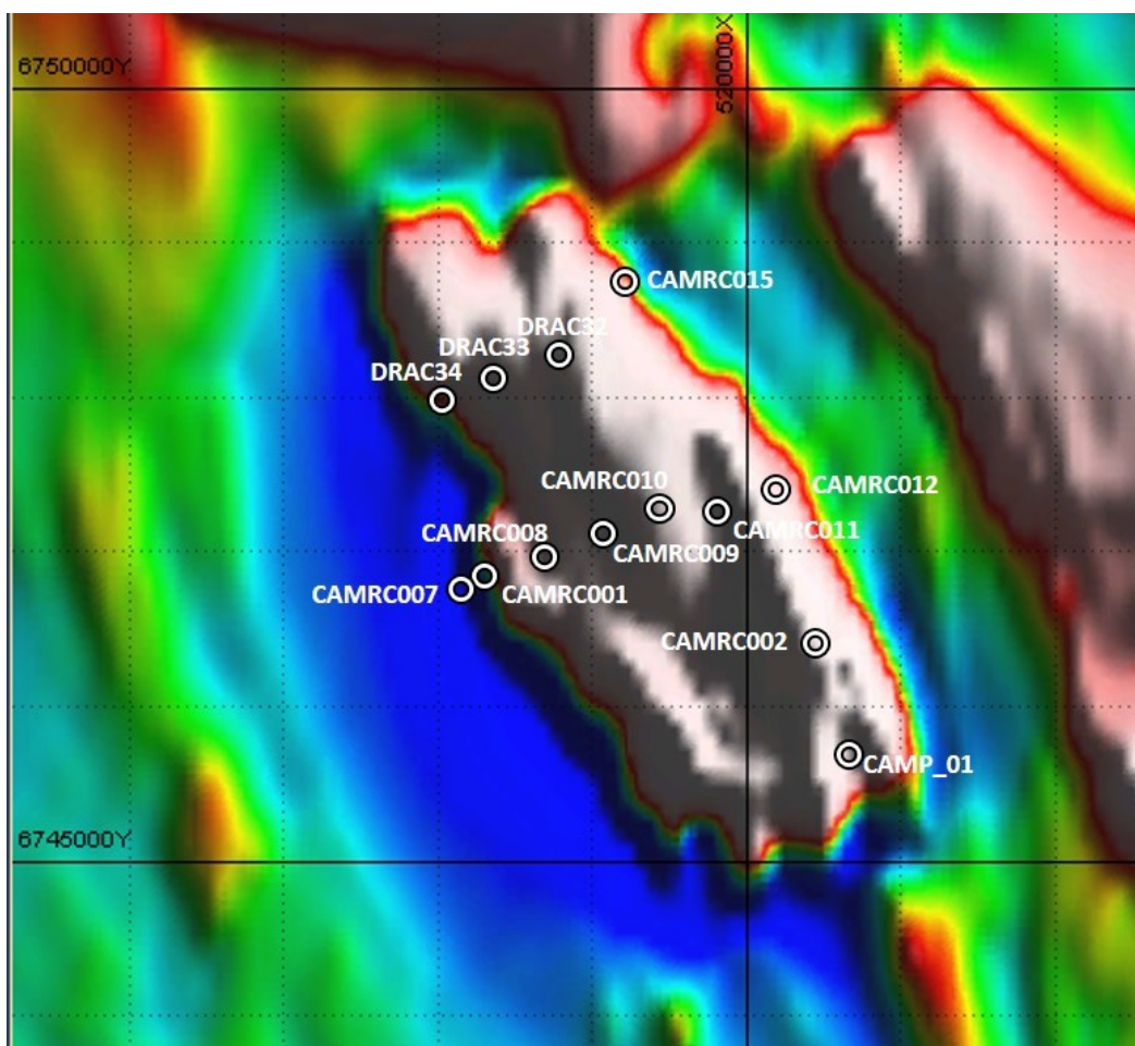
Figure 2 – A high-MgO zone has been identified along the eastern ridge of the large dunite body at Cambridge. The deep drill hole planned at CAMP_01 will test for nickel sulphide mineralisation below this prospective high-MgO zone.
