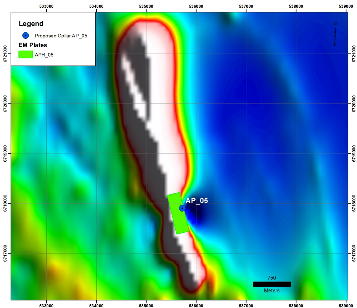
Figure 1 - Aphrodite 4, to be tested by planned drill hole AP_05, is situated in a pronounced indentation of the ultramafic body. This ‘embayment’ is a highly favourable site for the potential concentration of massive nickel sulphides.
