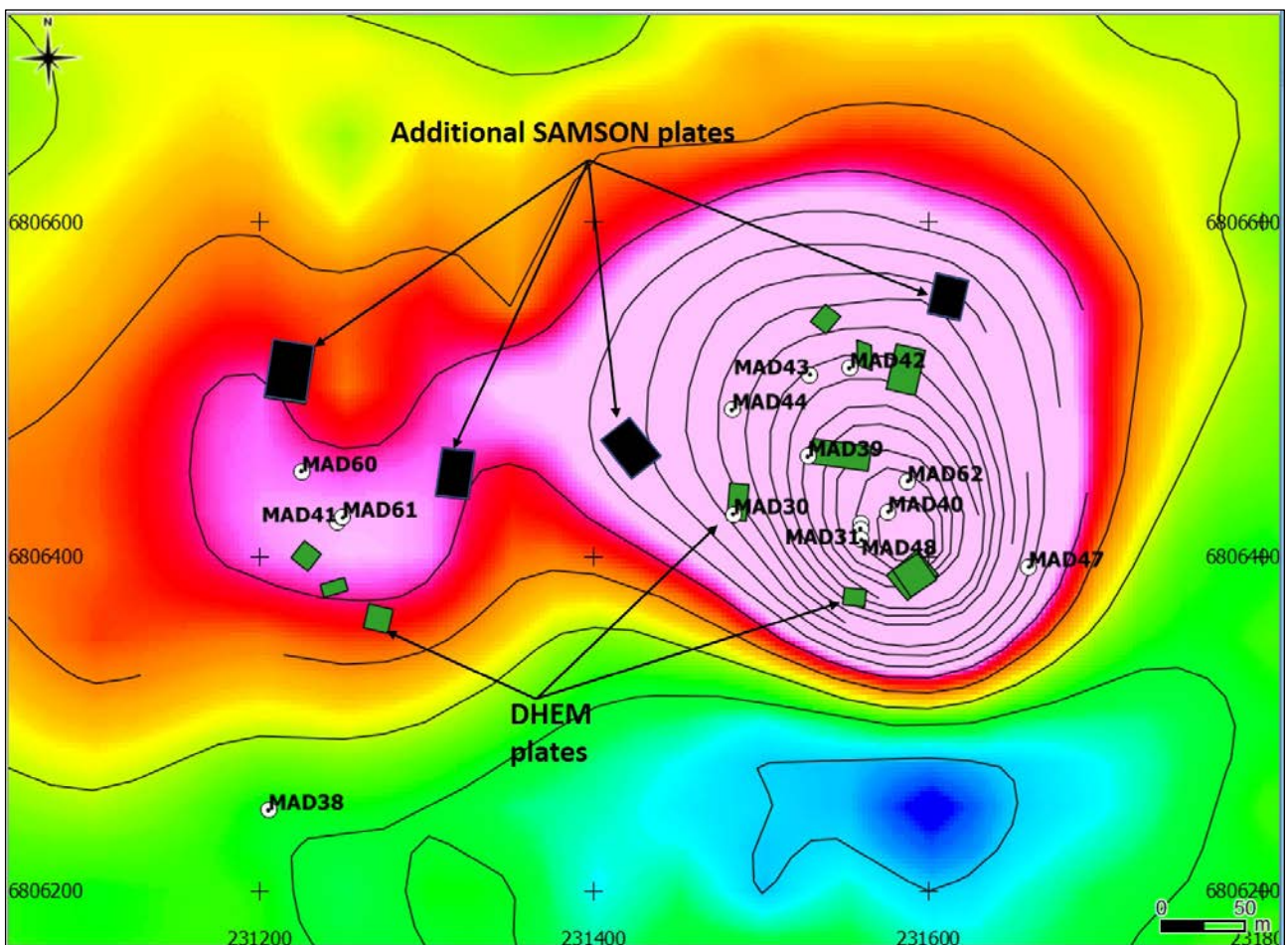
Figure 1 – a plan view of the Investigators Prospect showing the large SAMSON total field EM anomaly (in purple) in Channel 18 (44ms) in the eastern and central parts of Investigators. The contours shown are 0.05pT/A which highlight areas of stronger electromagnetic conductivity. Drill holes from the recent programme are shown together with untested SAMSON EM plates and DHEM plates.
