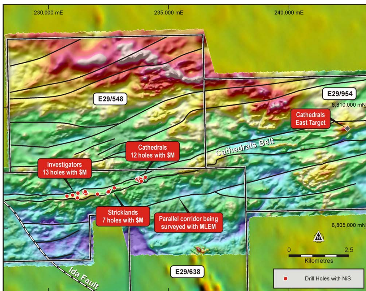
Figure 3 – a map of the Cathedrals Belt (against high resolution Total Magnetic Intensity) showing the multiple intersections of massive nickel-copper-cobalt-PGE sulphides (“$M”) at Investigators, Stricklands and Cathedrals which have established recurrent high grade mineralisation over a strike length of 3.5km. The high resolution magnetic data is set against TMI RTP magnetics from regional GSWA aeromagnetic surveys.
