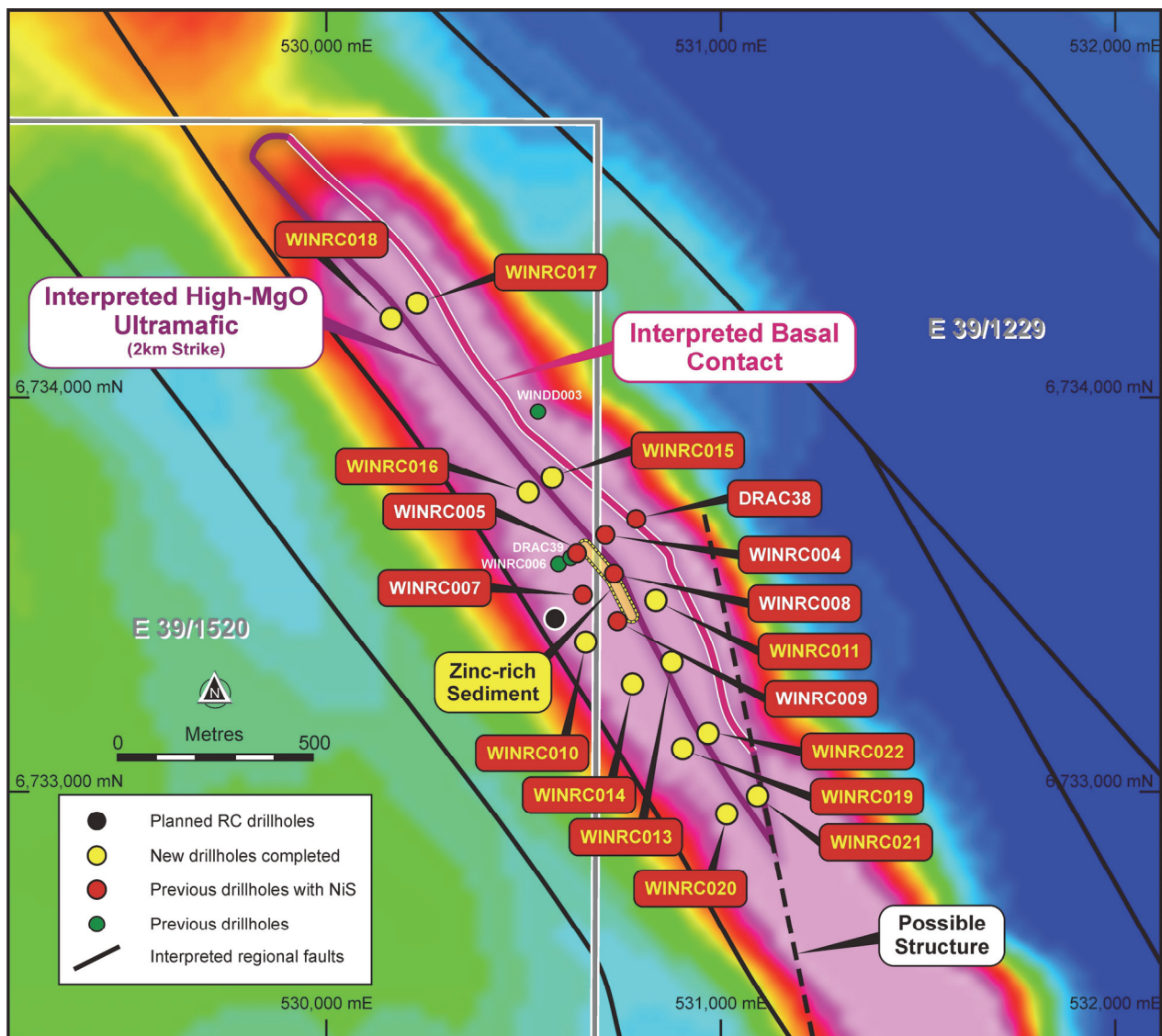
Figure 1 – interpreted ultramafic at Windsor against magnetics showing the successful nickel sulphide drill holes and the newly completed drill holes from the current drilling programme.
