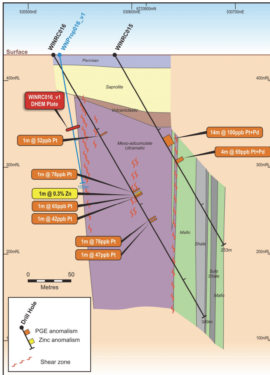
Figure 2 – Interpreted geological cross section of WINRC016 and WINRC015 (+/-50m), showing the prospective Windsor ultramafic with PGE intersections. The extremely conductive WINRC016_v1 plate is situated on the western contact of the Windsor ultramafic and will be tested by the planned hole shown.
