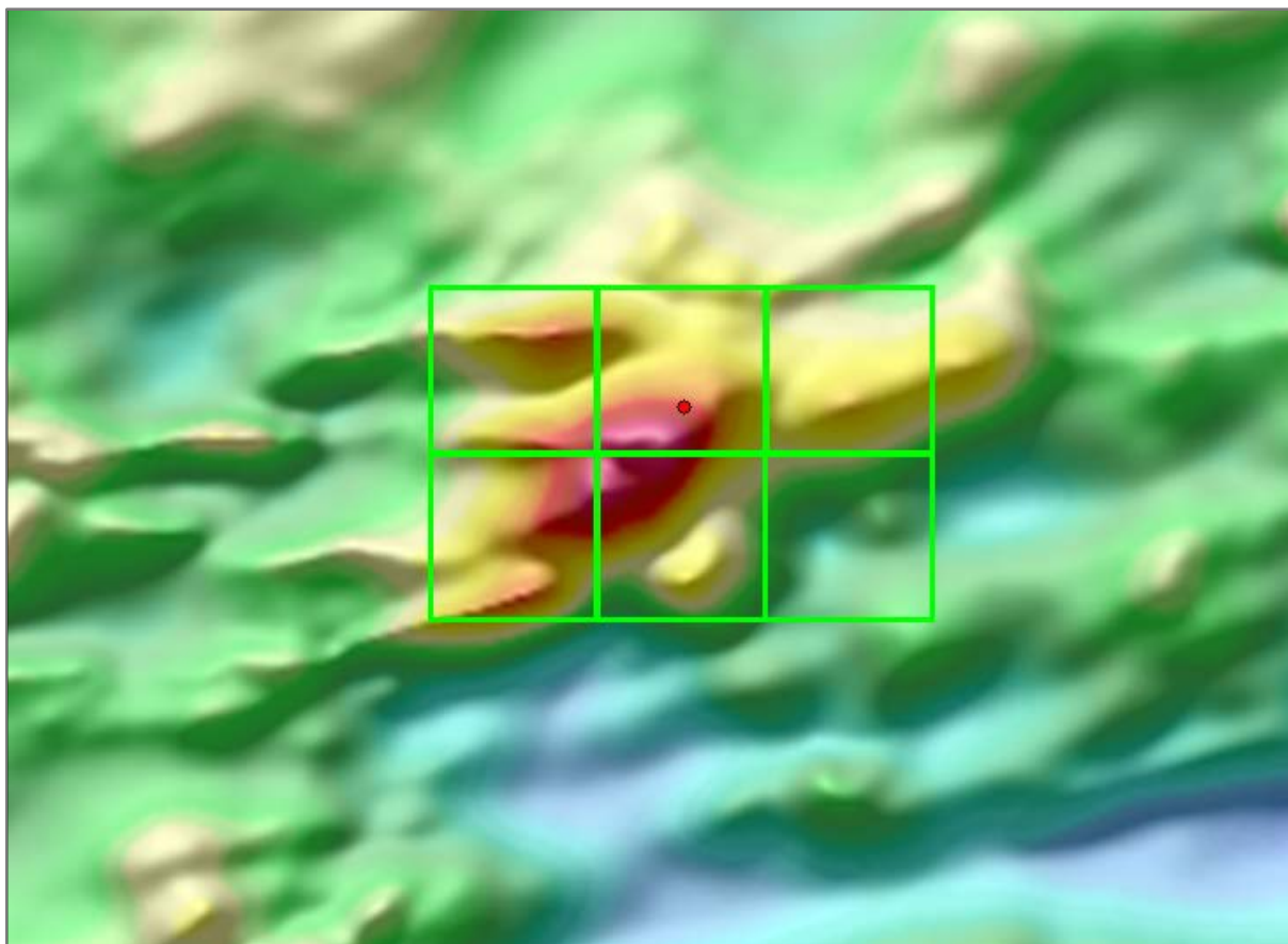
Figure 2 – the Cathedrals East target (against RTP magnetics) showing the FLEM and FREM survey loops. MAD64 is designated by the red dot, and was drilled to test a SAMSON anomaly that is on the northern edge of a prominent magnetic anomaly.
