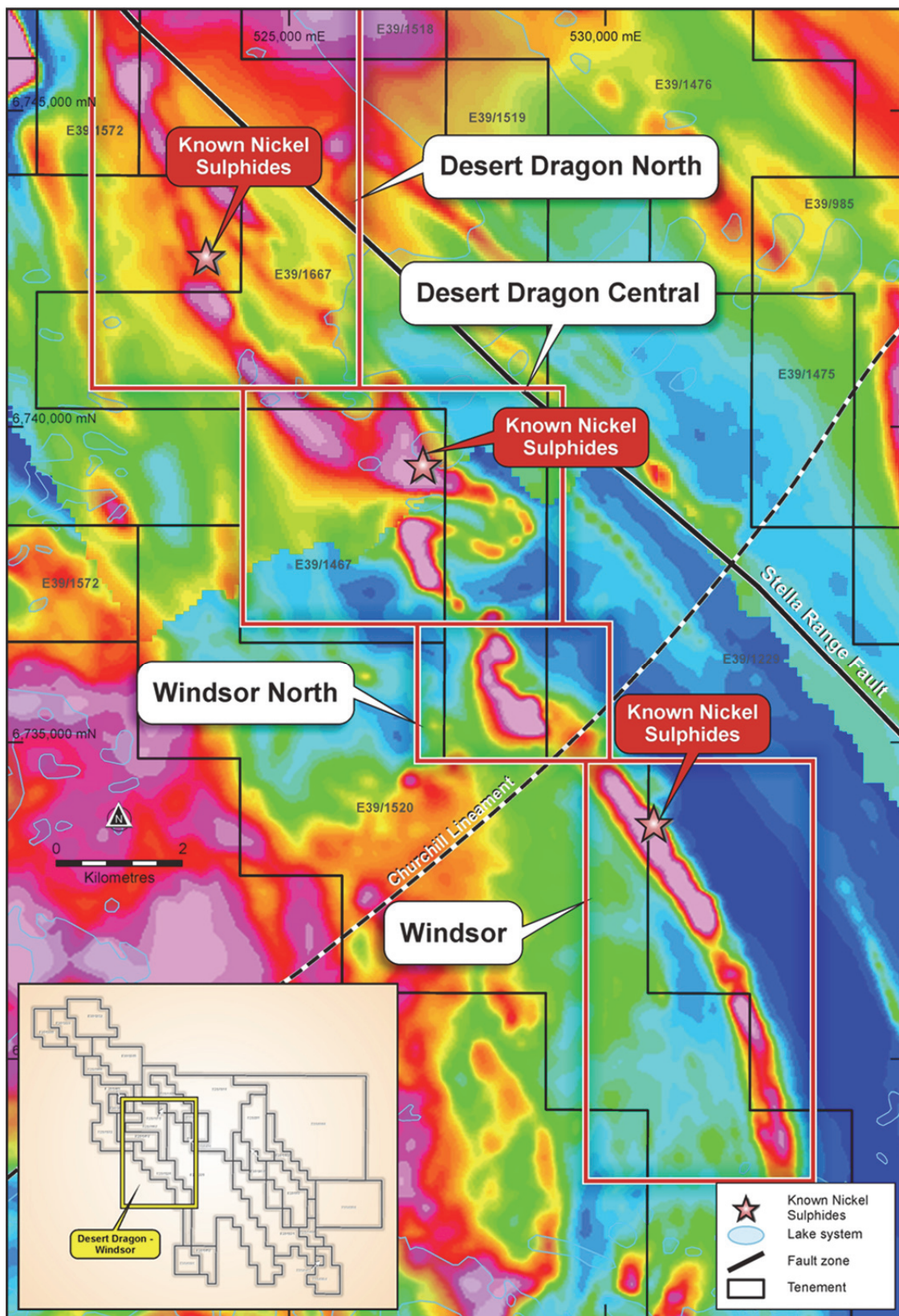
Figure 2 – the Windsor North prospect is within a priority 18km section of the Stella Range belt (the inset shows the location of this priority section within the tenement package at the East Laverton Project). Drilling in the current campaign commenced at Windsor. Windsor North will be the next target to be drilled, following which the drill rig will move northwards to Desert Dragon for testing of EM conductors in favourable geological positions.
