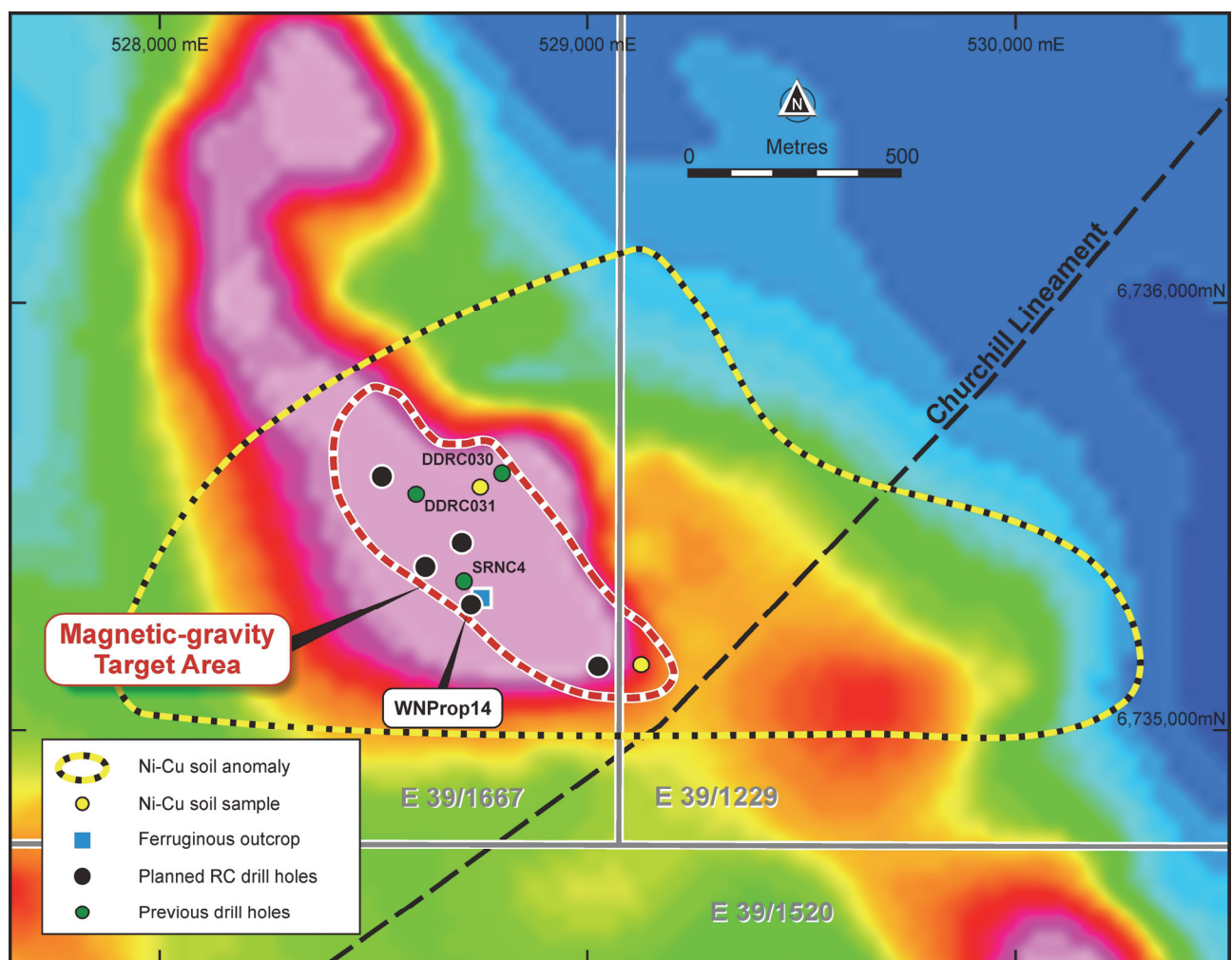
Figure 1 – plan view of Windsor North against TMI magnetics. Historical drill holes and the planned drilling by St George are highlighted as well as the co-incident Ni-Cu soil anomaly and the two high value samples within the target area.
