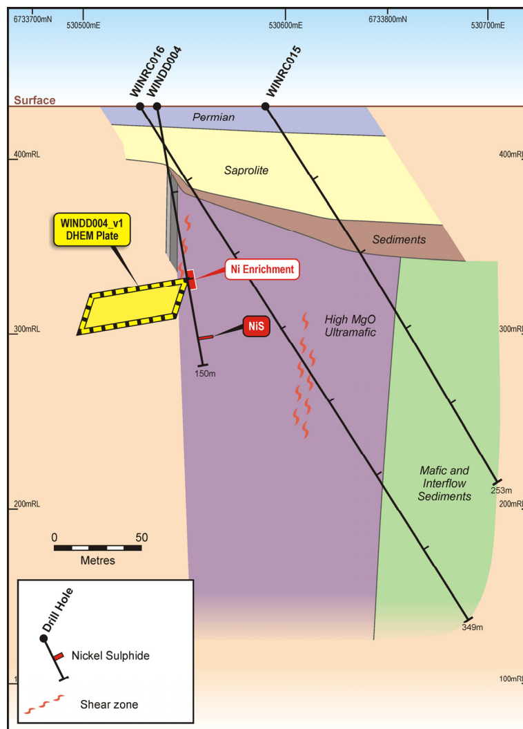
Figure 1 – Interpreted geological cross section of WINDD004, WINRC016 and WINRC015 (+/-50m) showing the WINDD004_v1 plate on the western contact of the Windsor ultramafic.
