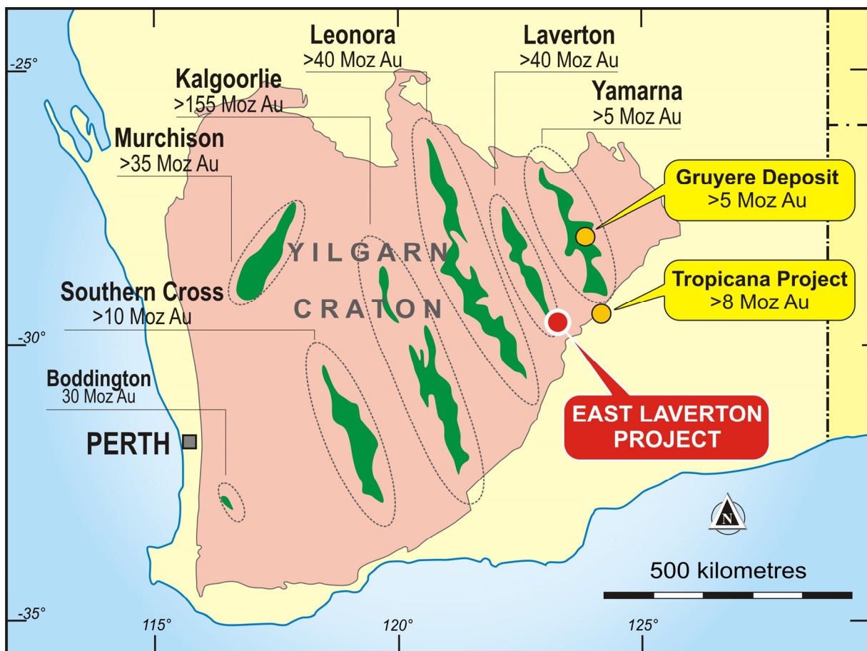
Figure 4 – the main gold-bearing greenstone belts of the Yilgarn Craton, a world class gold province with an endowment of over 300 million ounces of gold. The East Laverton Project is in the eastern margin of the Yilgarn Craton, where major new discoveries continue to be made.
