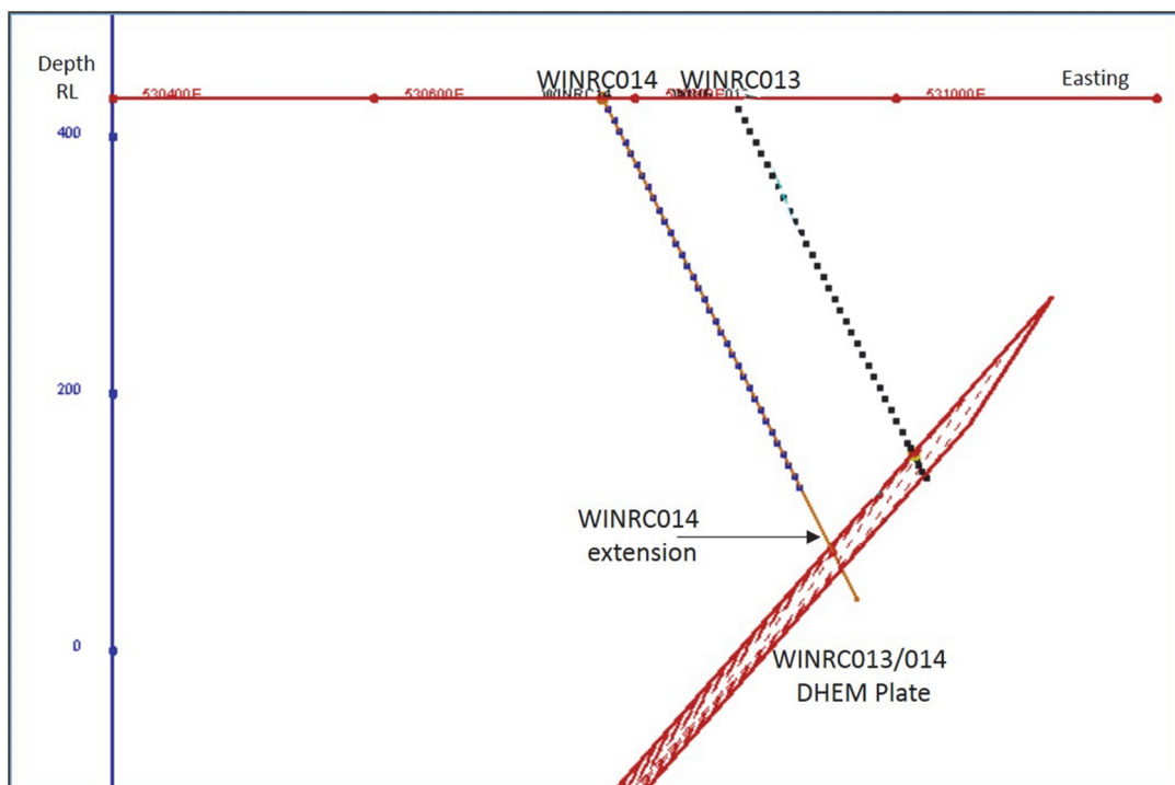
Figure 1 – the modelled DHEM plate for the off-hole conductor to be tested by the extension of WINRC014. WINRC013 did not intersect the conductor.
